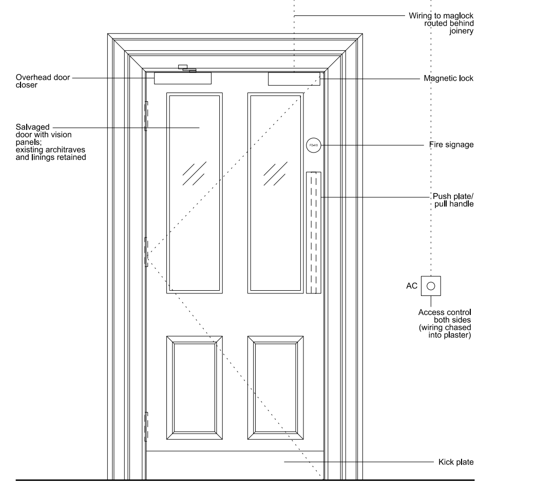
09 144/D3n - Plan and External Elevation
