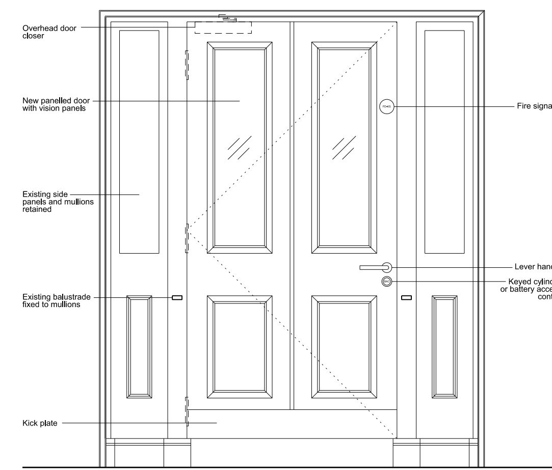
02 201/D1n - External Elevation
