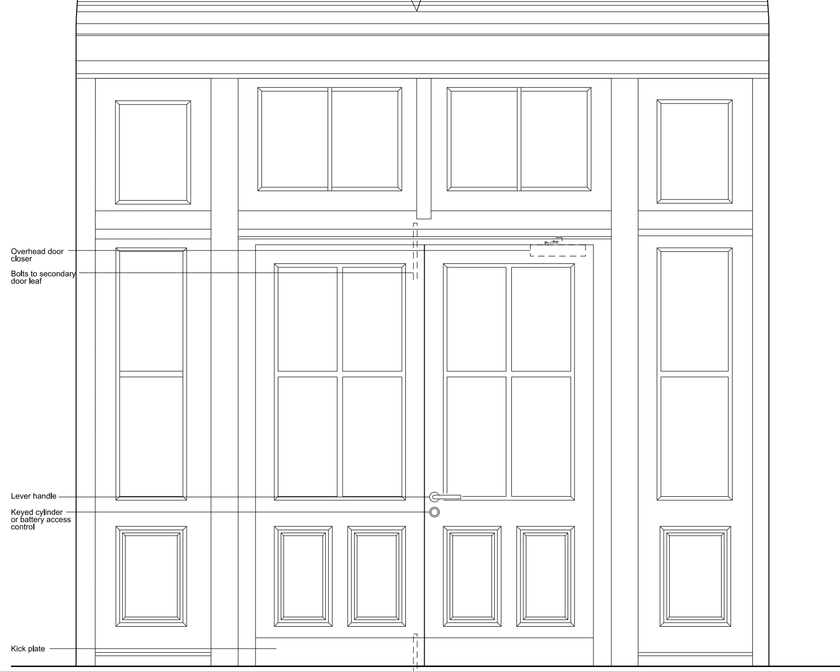
08 142/D1n - Plan and External Elevation
