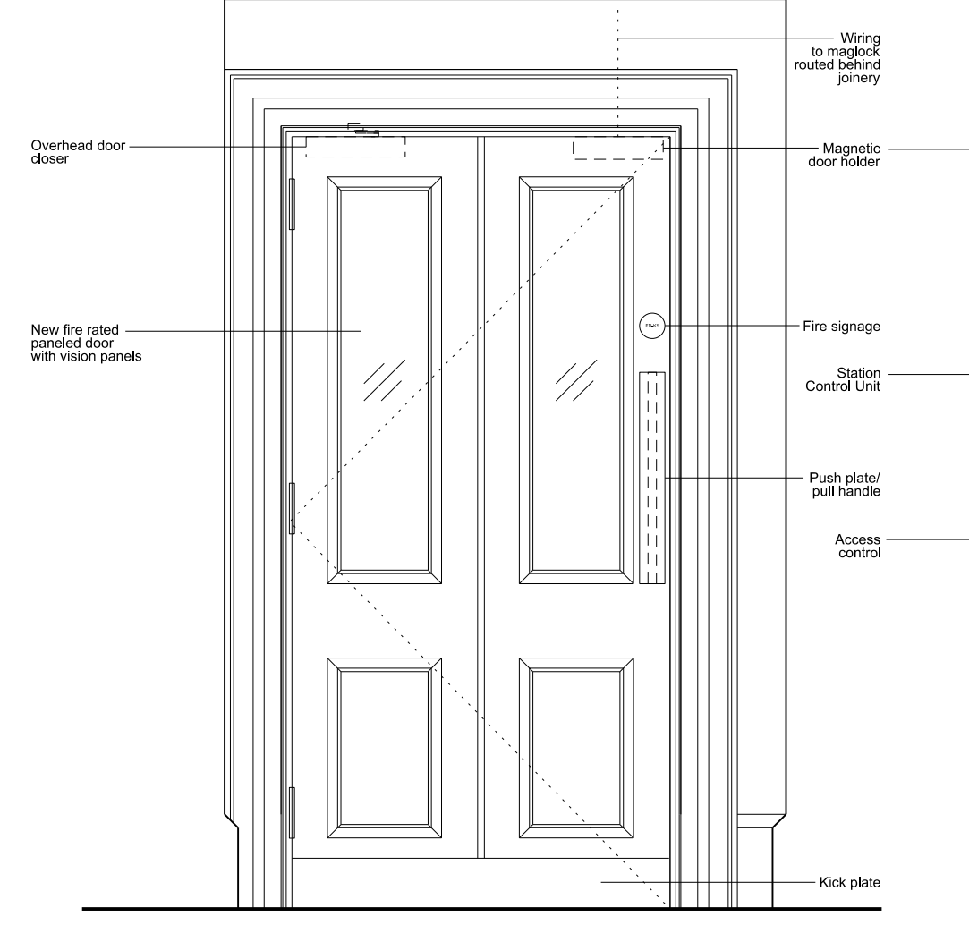
03 107/D1n - External Elevation
