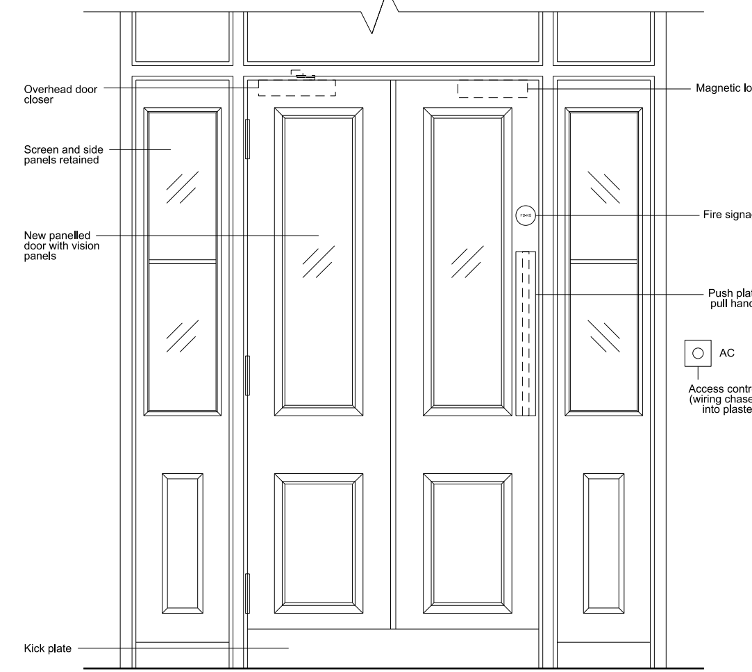
03 107/D1n - External Elevation
