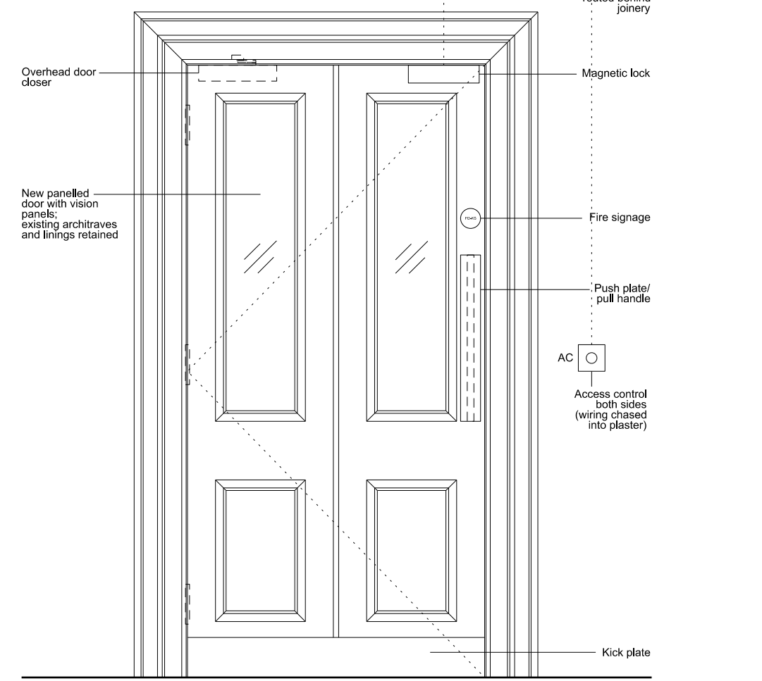
04 207/D1e - External Elevation
