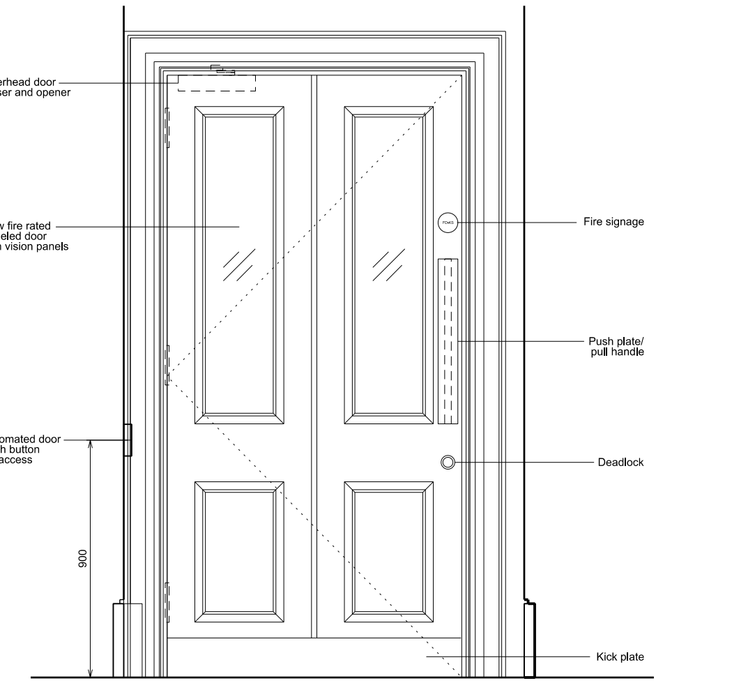
02 201/D1n - External Elevation
