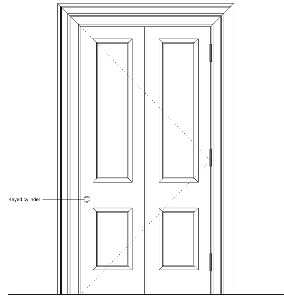
05 Reeded door fixed shut (Non reeded door as detail 03 with ironmongery as this detail)
