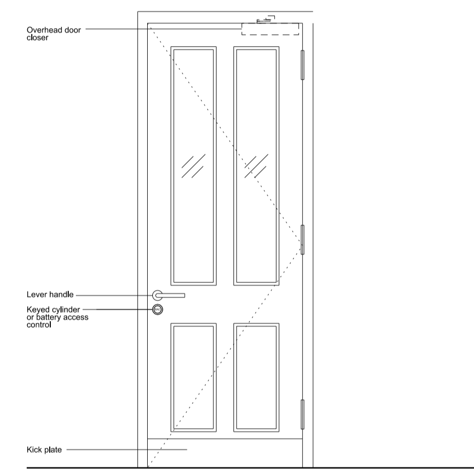
07 317/D1e - External Elevation
