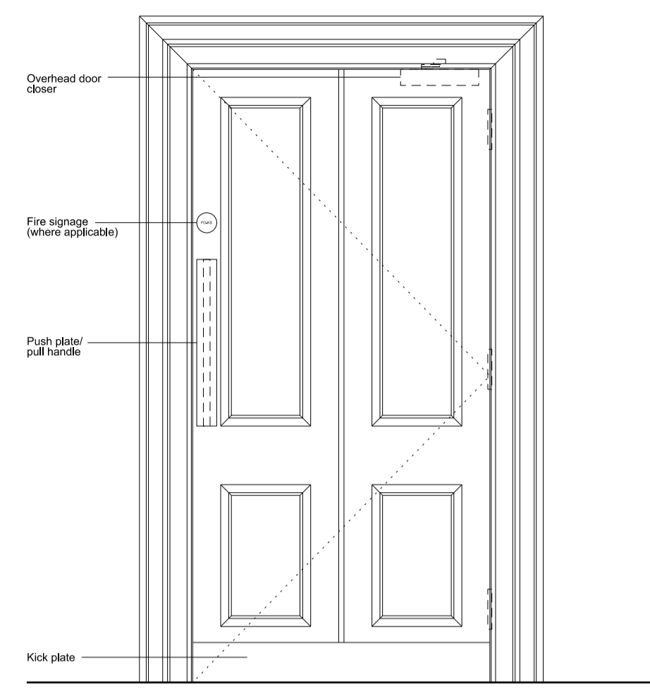
02 Typical reeded door with pull handle/push plate
