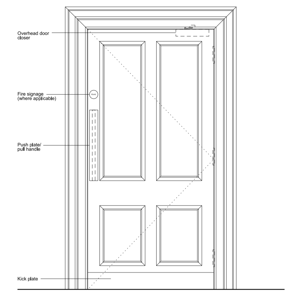
04 Typical paneled door with pull handle/push plate
