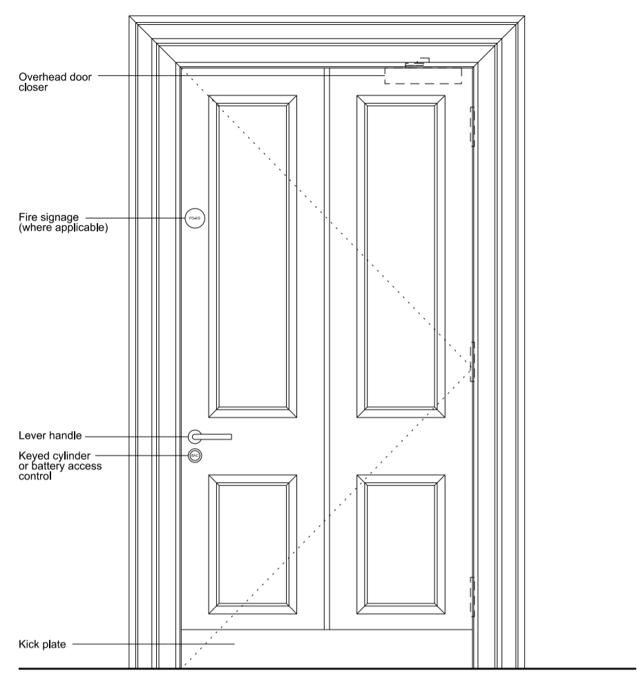
01 Typical reeded door with lever handle
