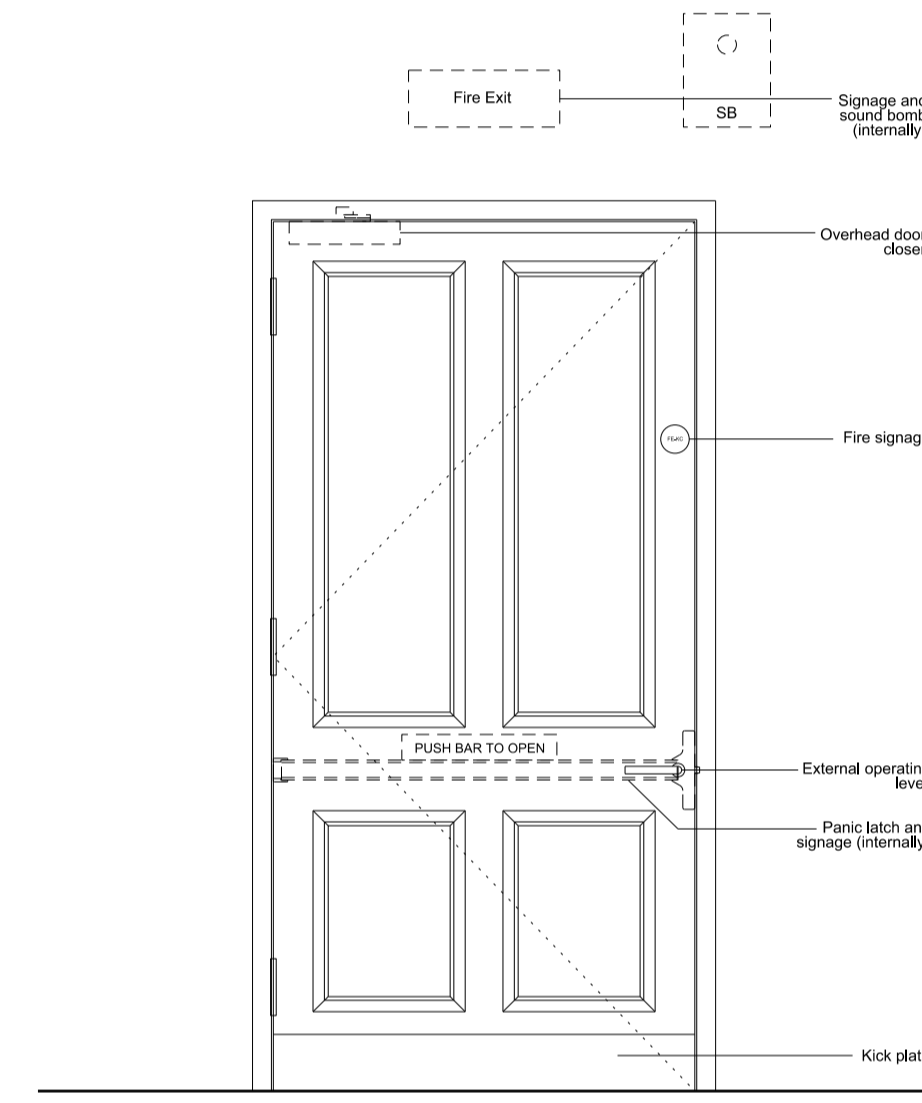
06 Typical external paneled door with panic hardware
