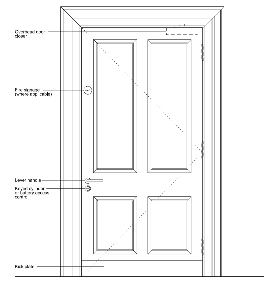
03 Typical paneled door with lever handle
