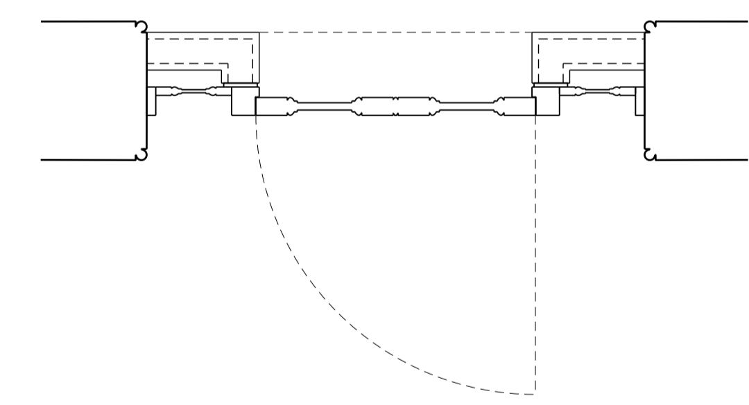
08 G19/D2n - Elevation and Plan
