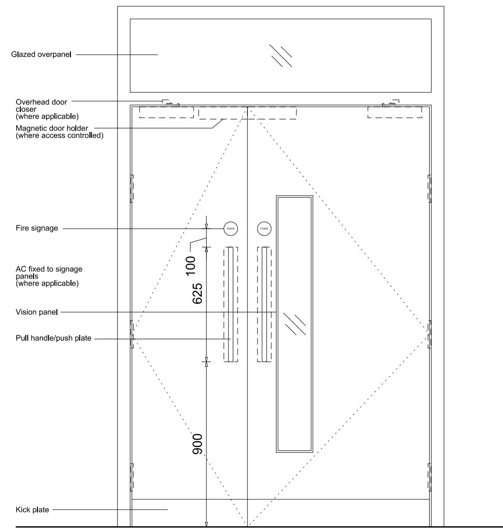
01 Typical 1.5 leaf corridor door
