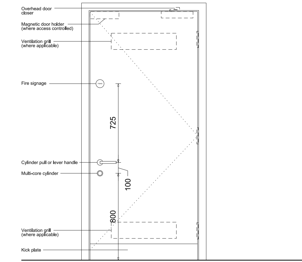
04 Typical single leaf door
