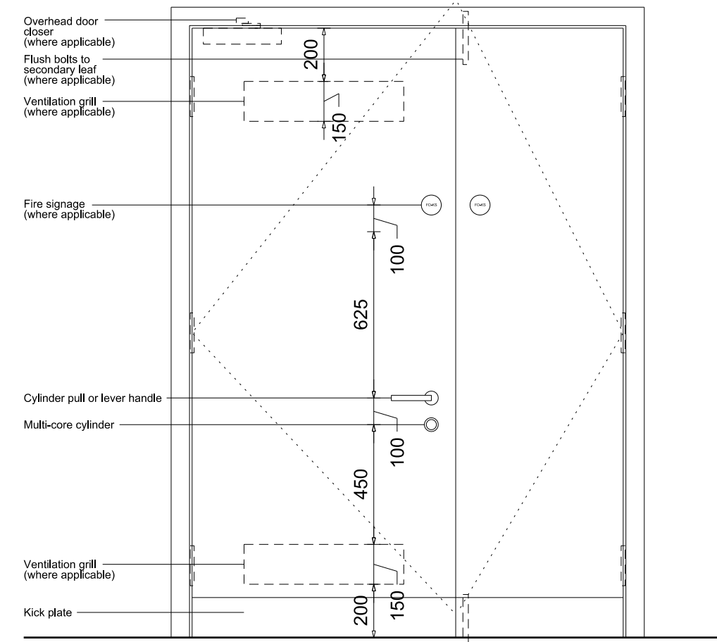
03 Typical 1.5 leaf door
