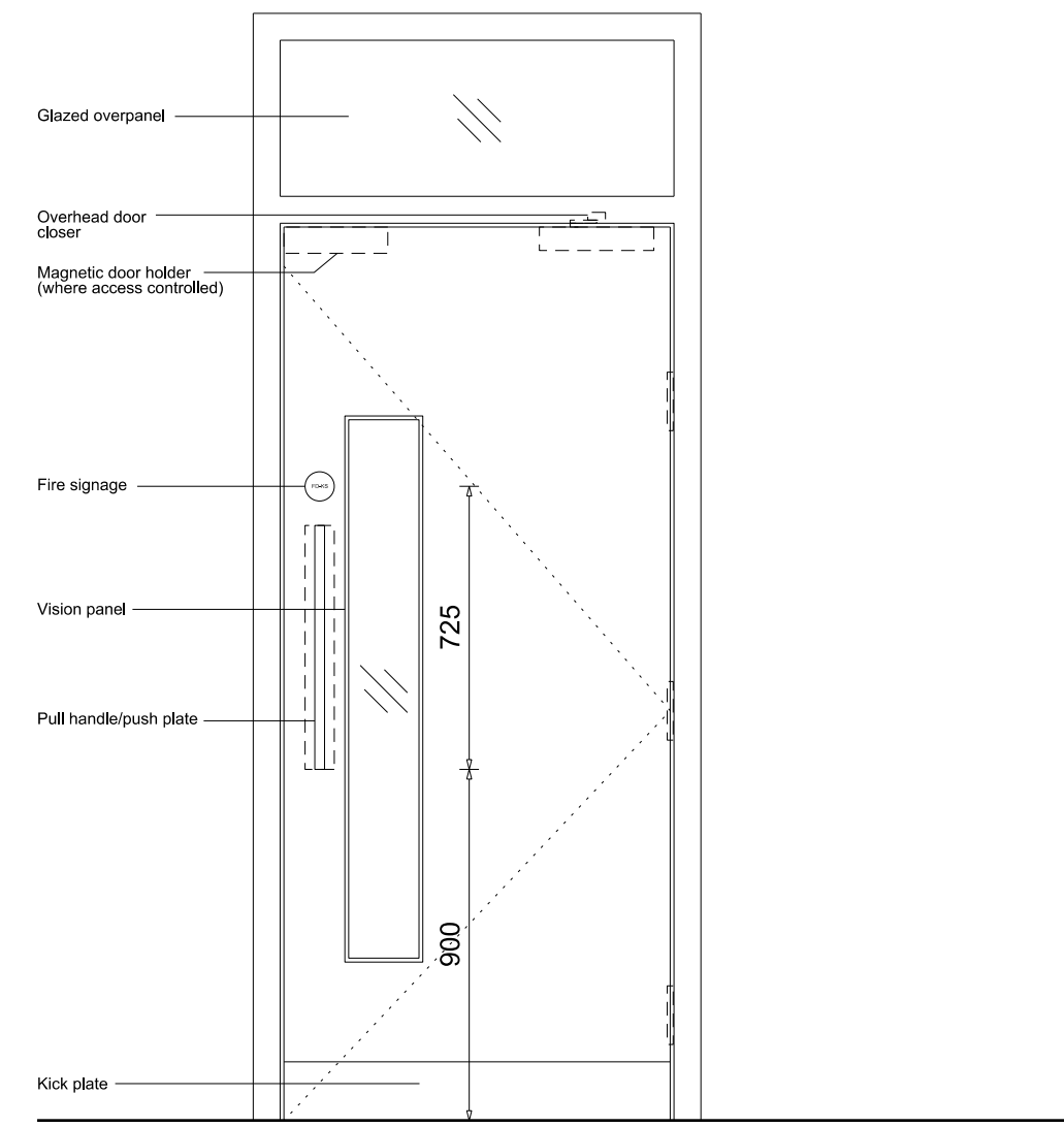
02 Typical single leaf corridor door
