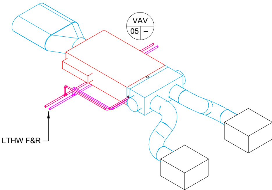
Typical VAV connection detail (NTS)
