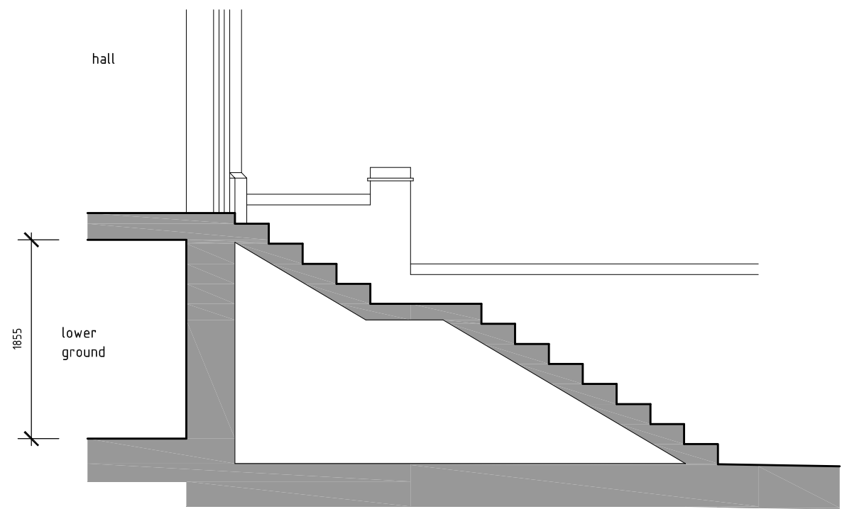
FRONT STEPS SECTION C-C (AS EXISTING)
