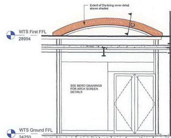
3 Arch type B interior elevation 1:50
