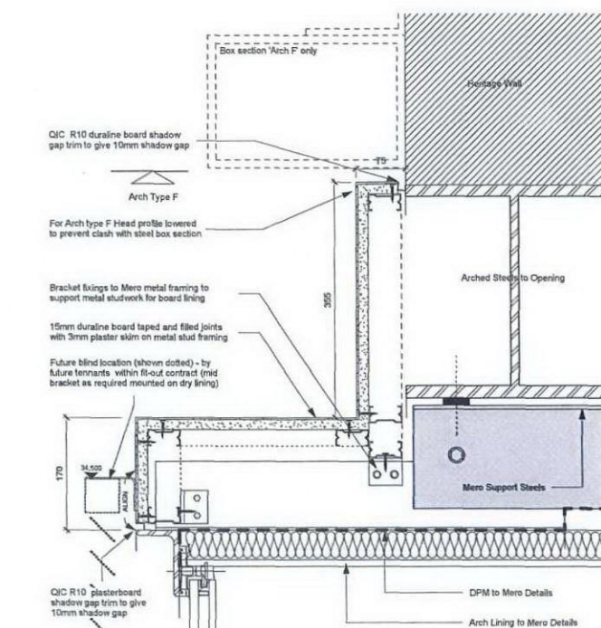
5 Section detail A-2 1:5
