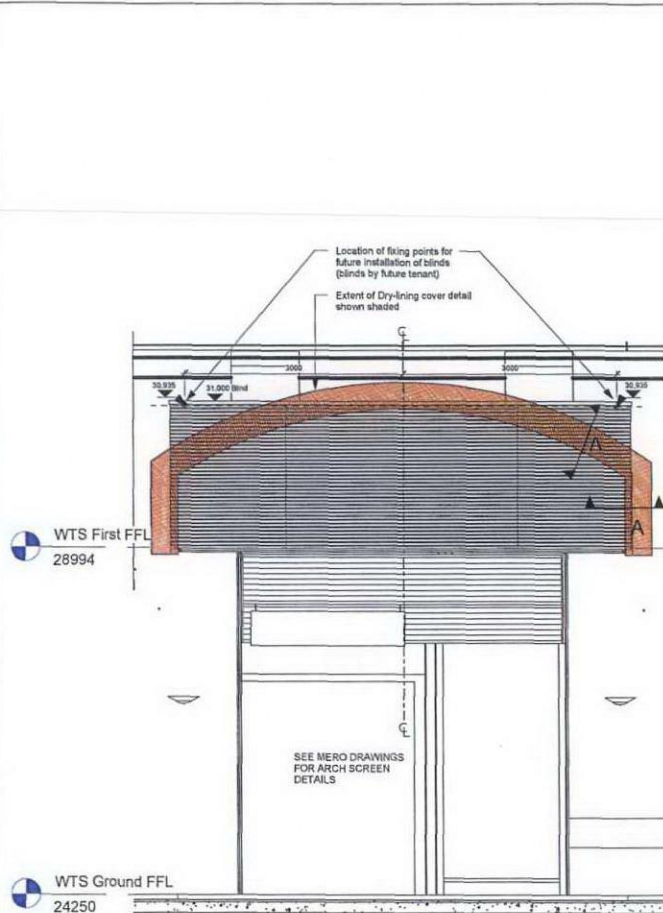
1 Arch type A/D interior elevation 1:50
