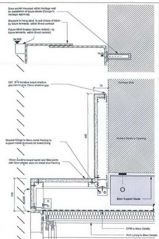
8 Section detail D 1:5
