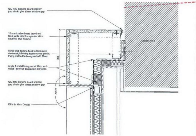
7 Section detail C 1:5
