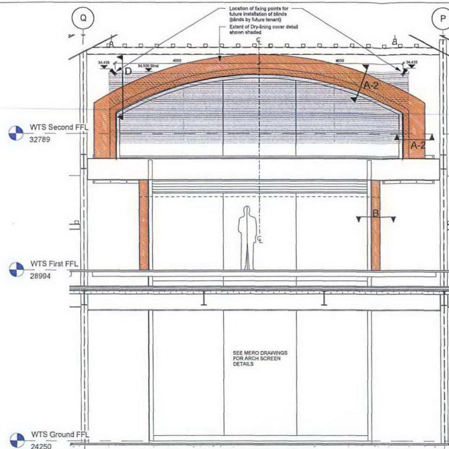
2 Arch type F interior elevation 1:50
