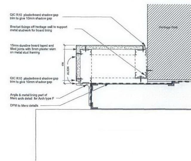
6 Plan detail B 1:5
