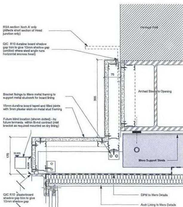
4 Section detail A 1:5
