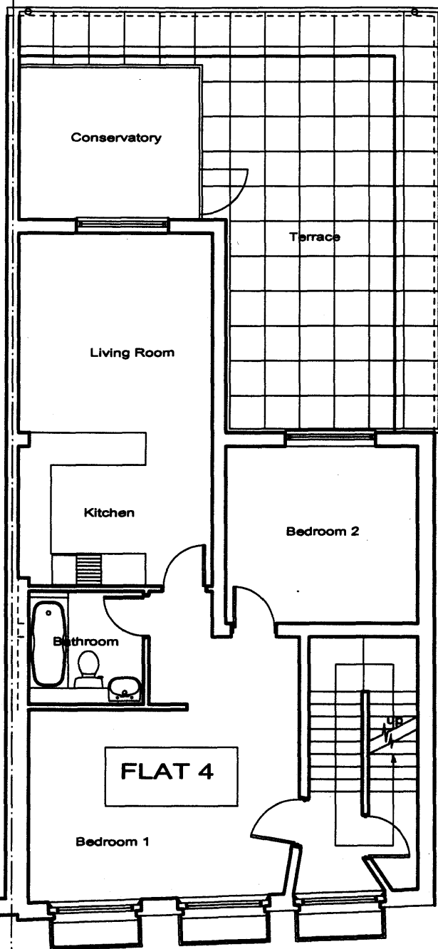
FIRST FLOOR
