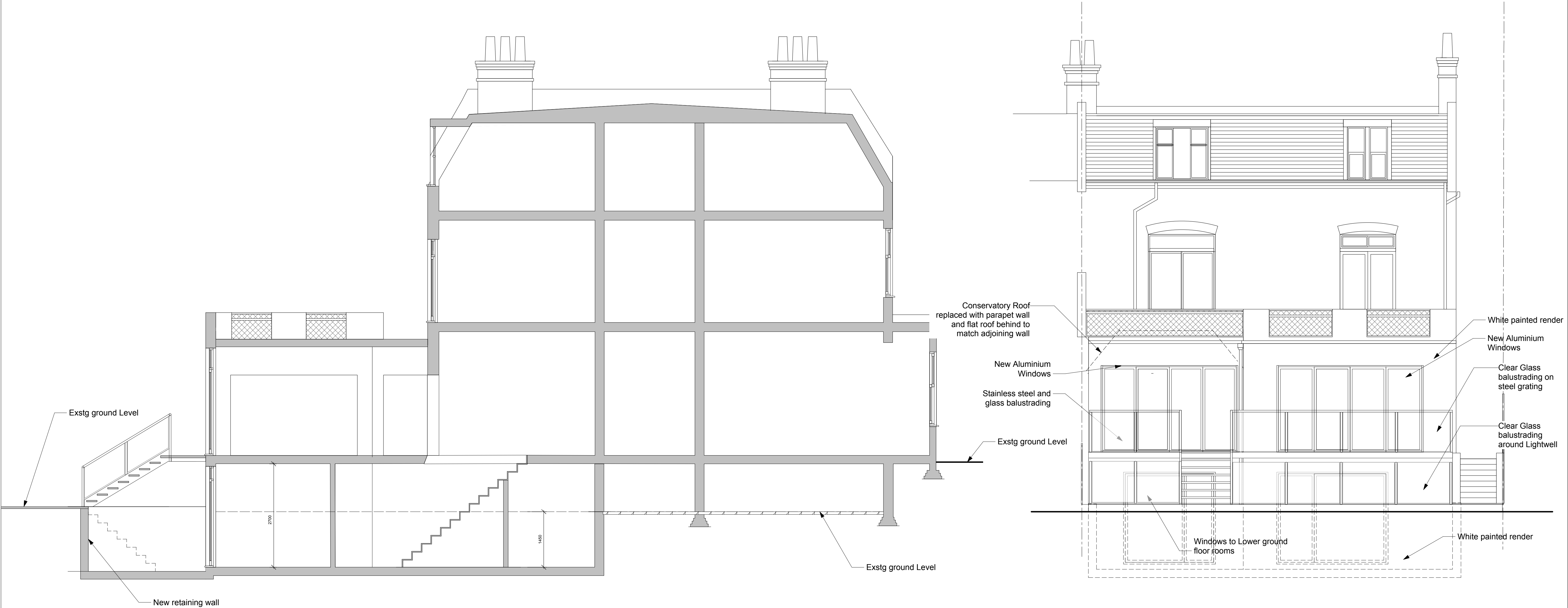
1 Proposed Section Looking West
