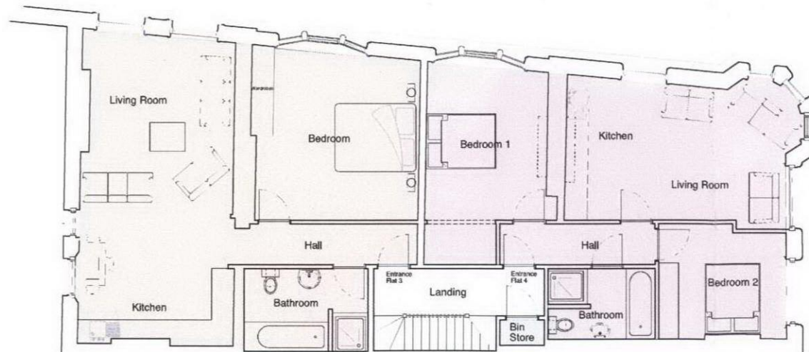
1 Second Floor Plan - Proposed Scale: 1:100
