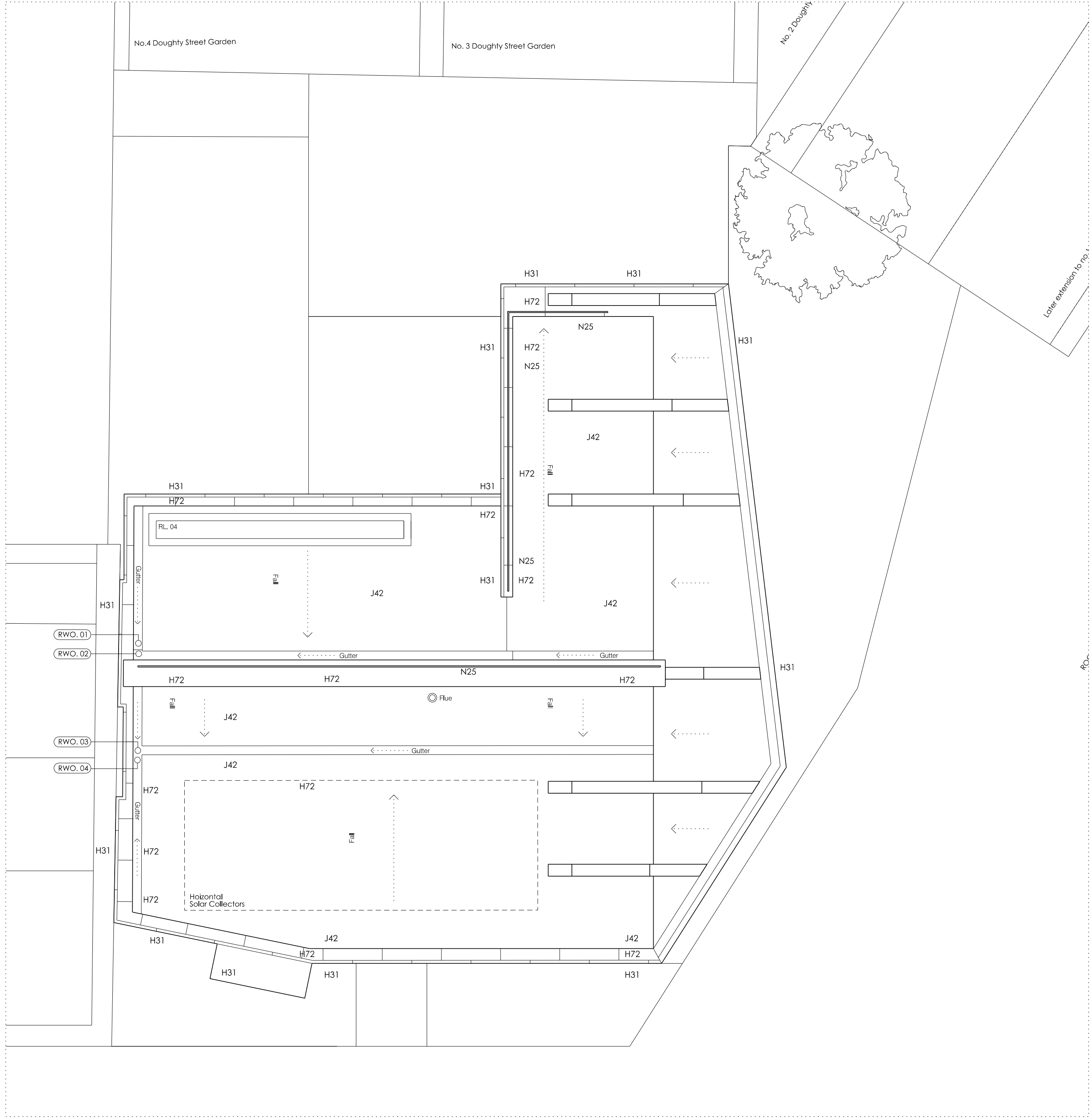
2 Roof GA Plan 104
