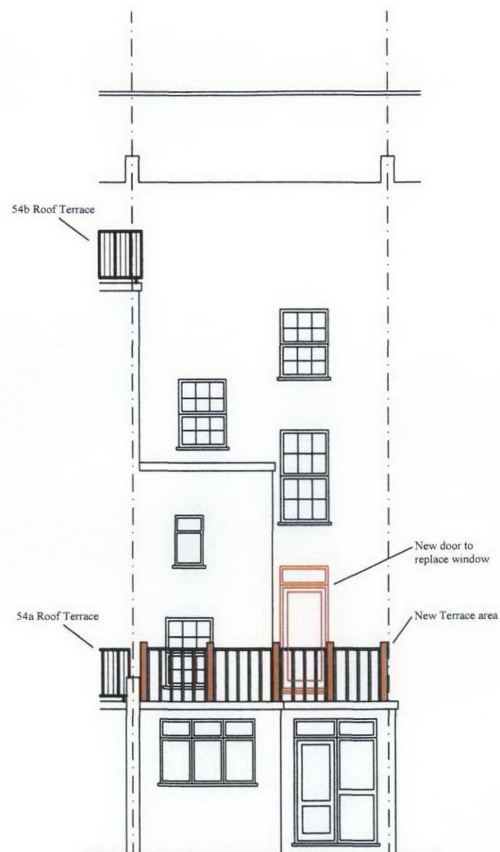
PROPOSED REAR ELEVATION (SOUTH)
