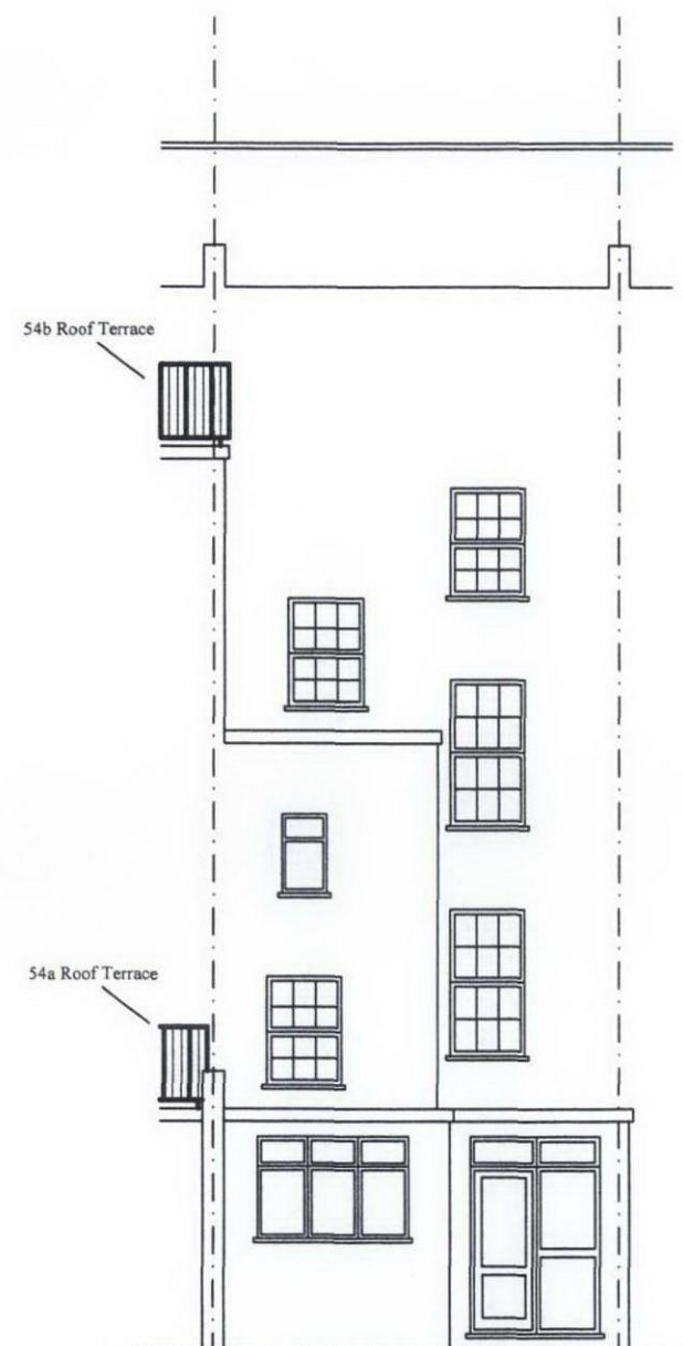
EXISTING REAR ELEVATION (SOUTH)
