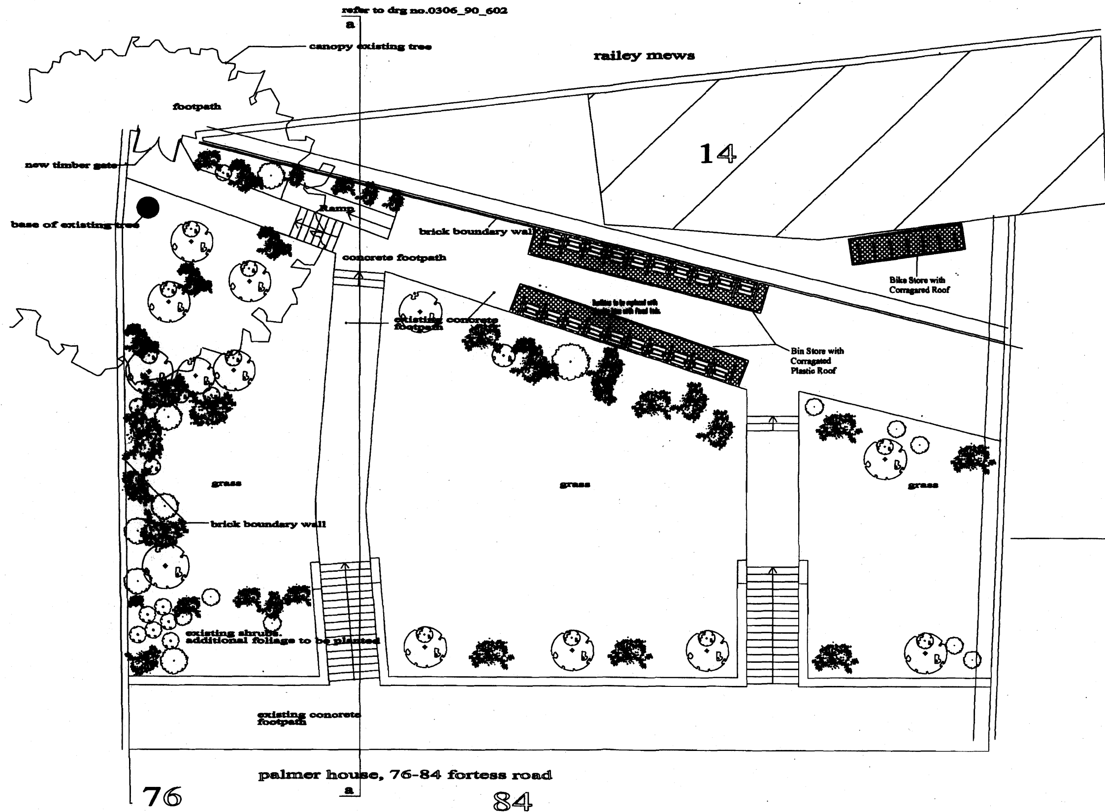
Palmer House Site Plan Proposed Bin and Bike Stores with Plastic Corroagated Roof Addition
