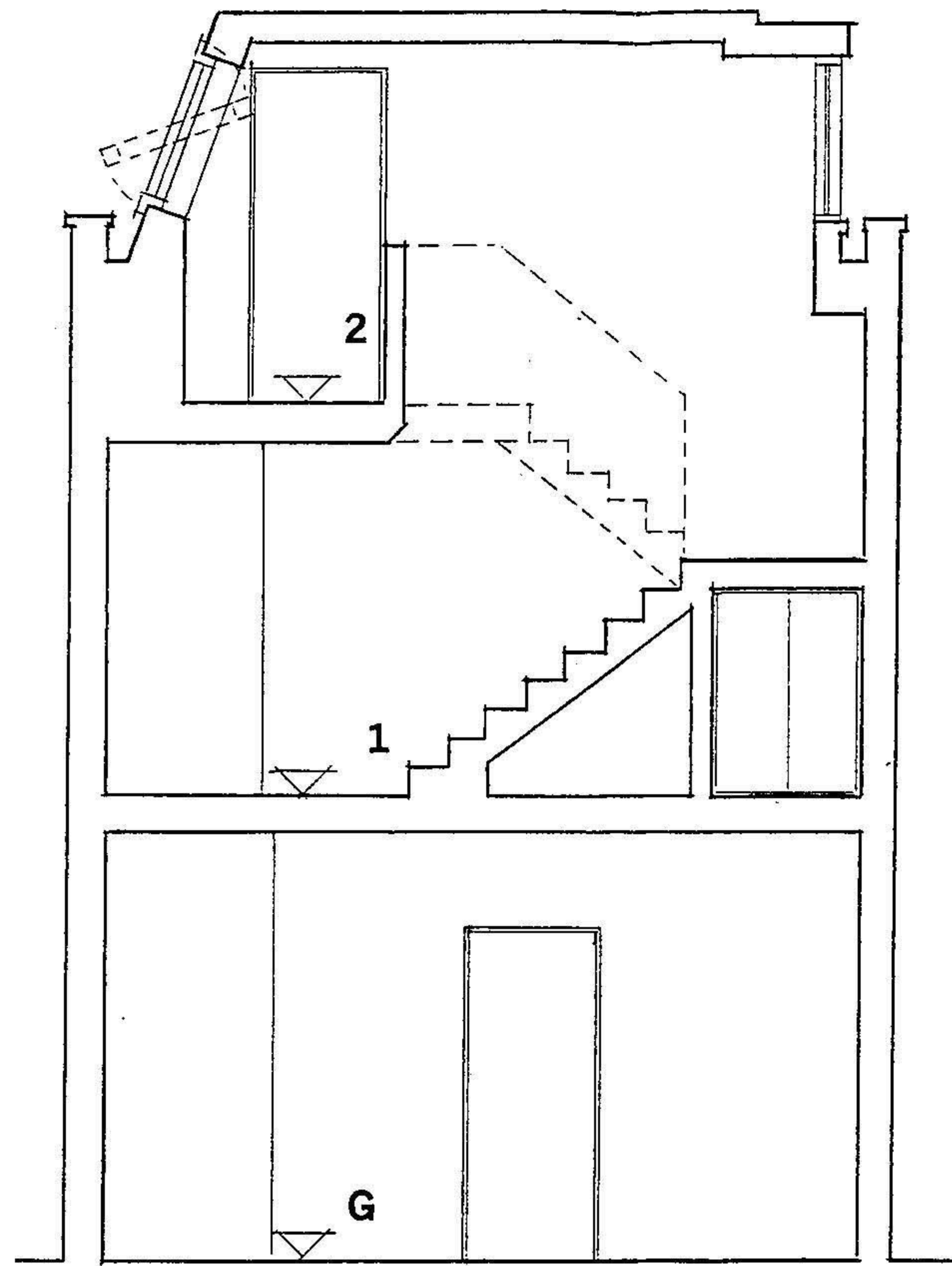
SECTION B-B
