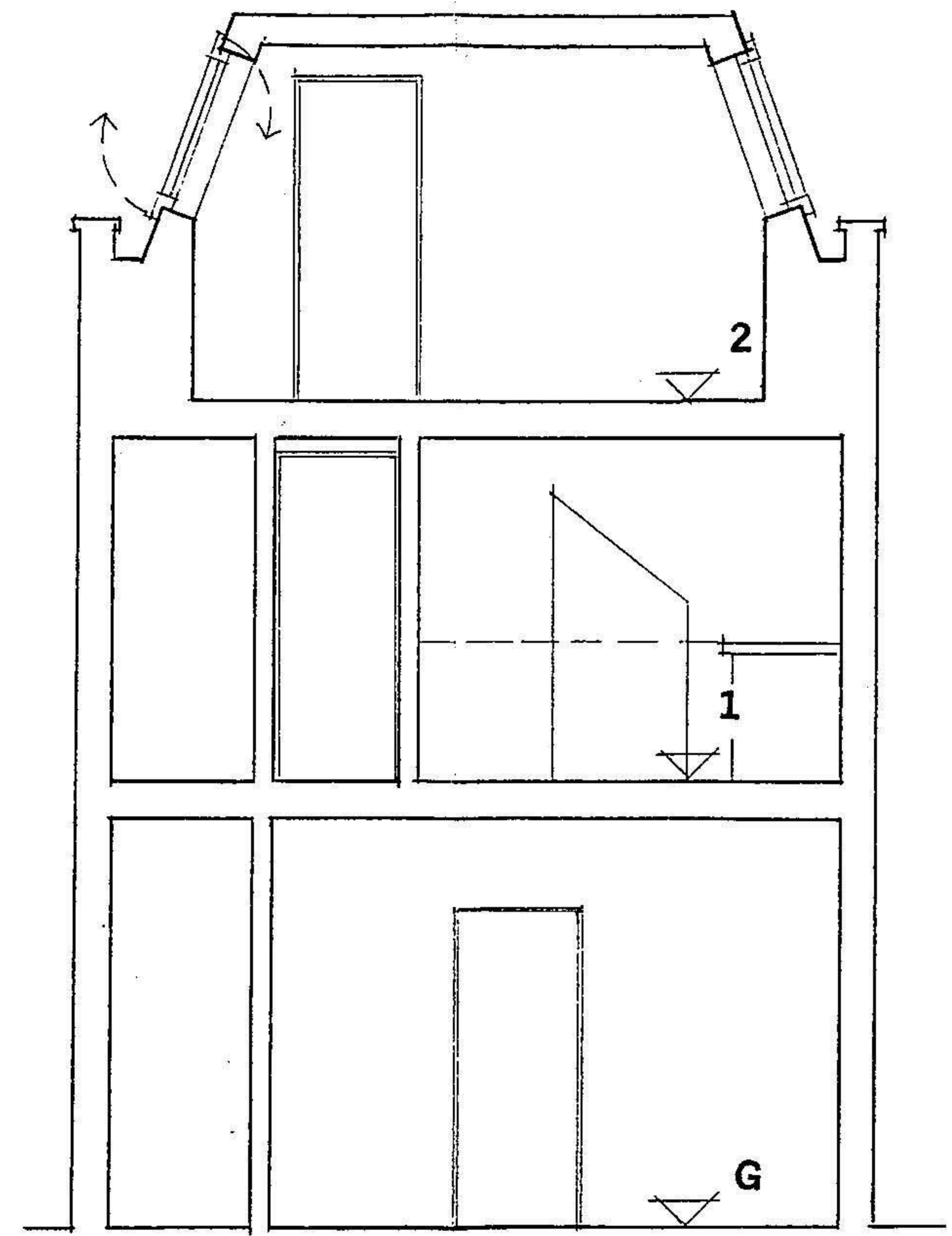
SECTION C-C
