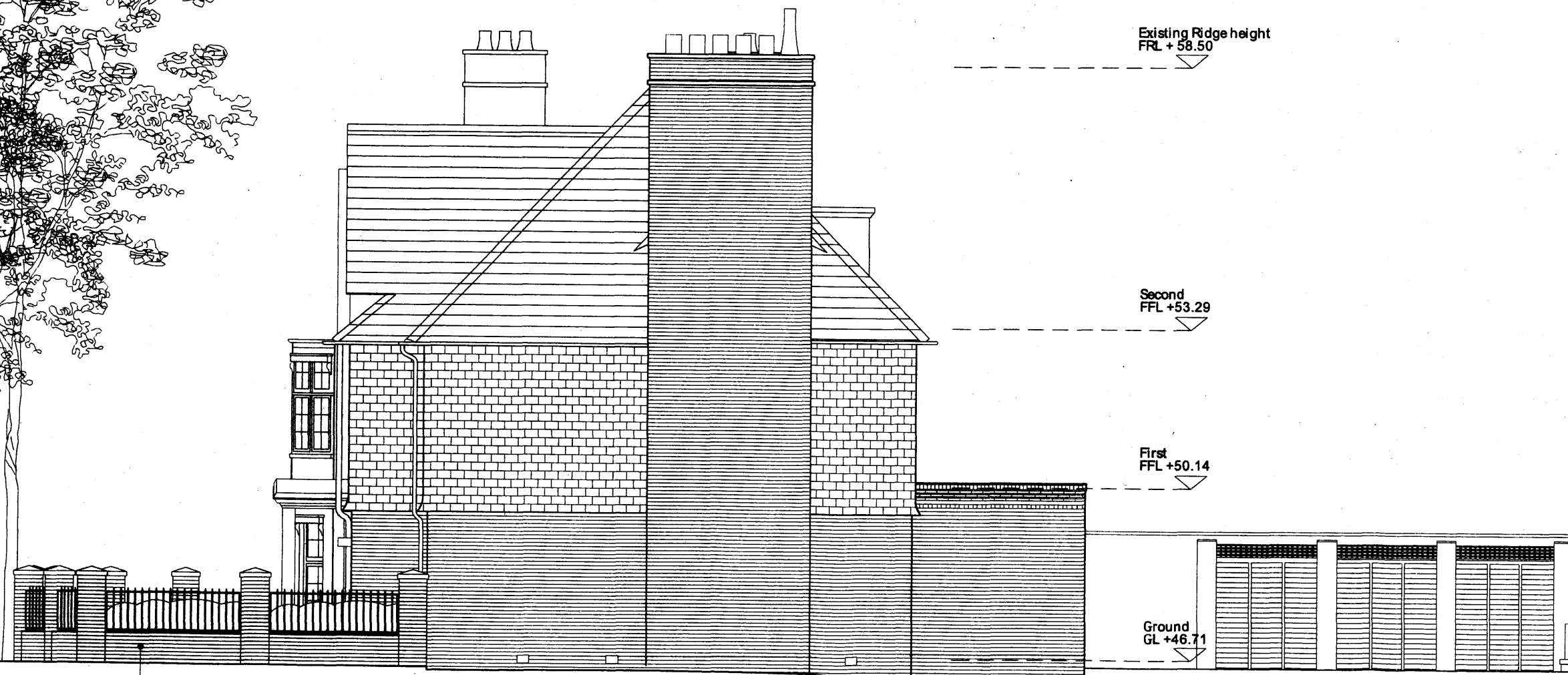
EAST/SIDE ELEVATION No 62 ELSWORTHY ROAD
