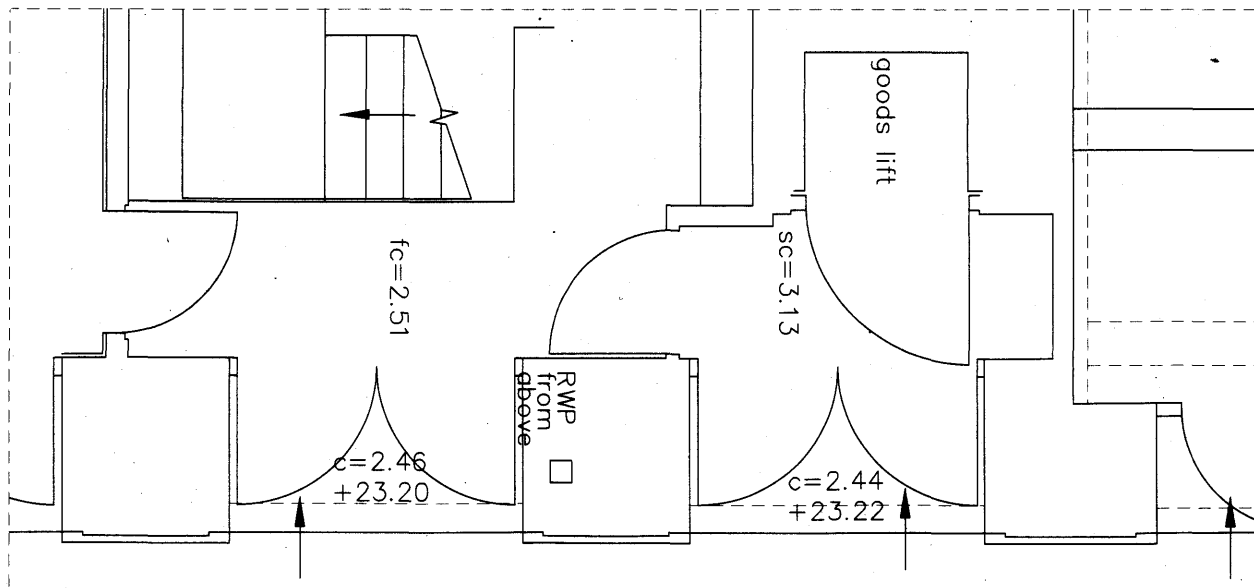
3 Existing Plan (1:50)
