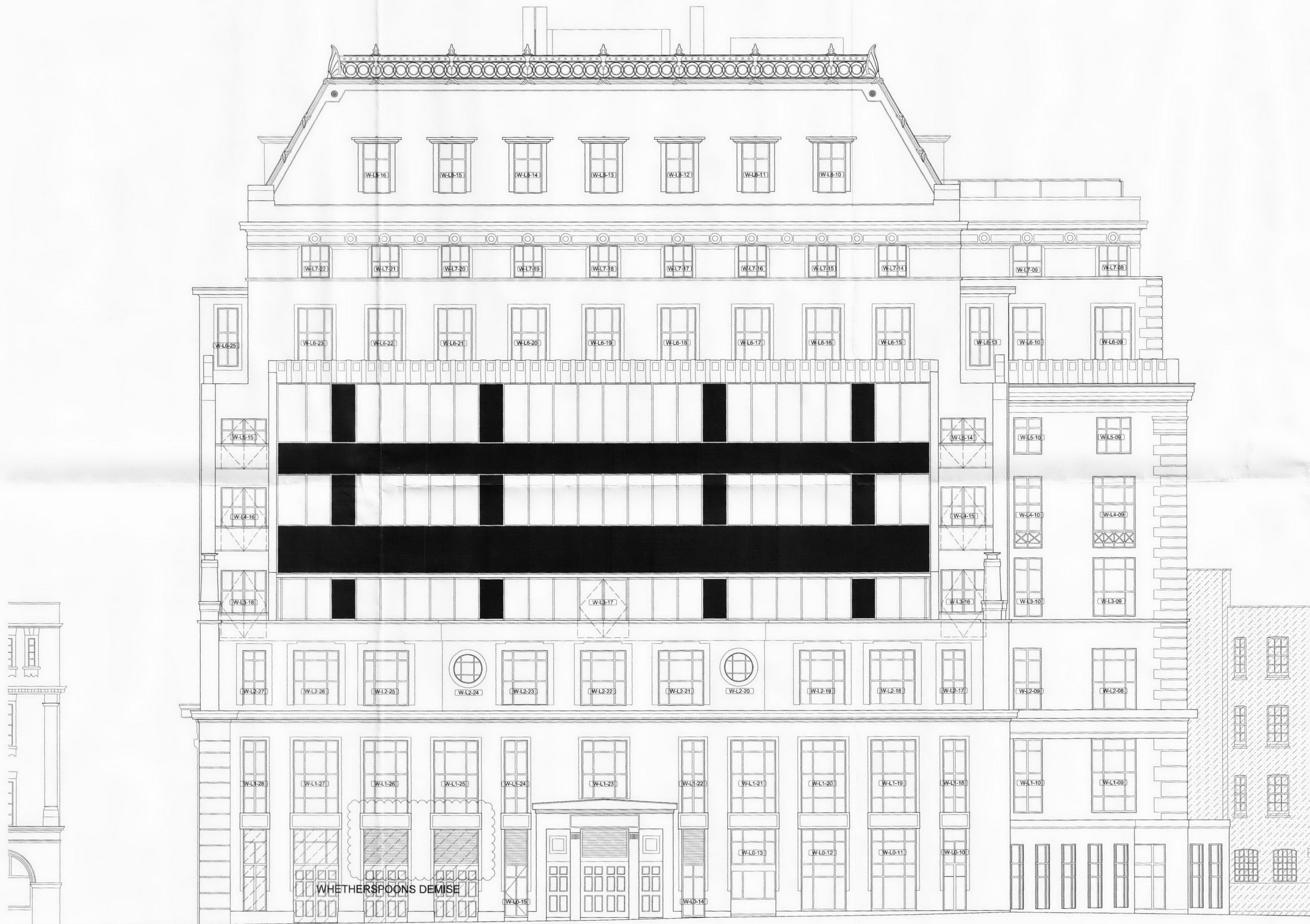
PROPOSED ELEVATION - EAST
