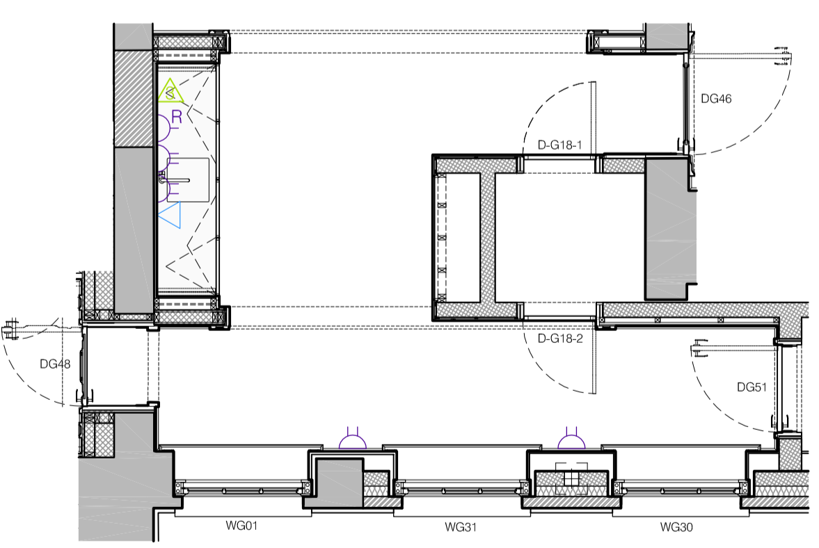
G18A SURVERY SMALL POWER PLAN Scale: 1:50 @ A1
