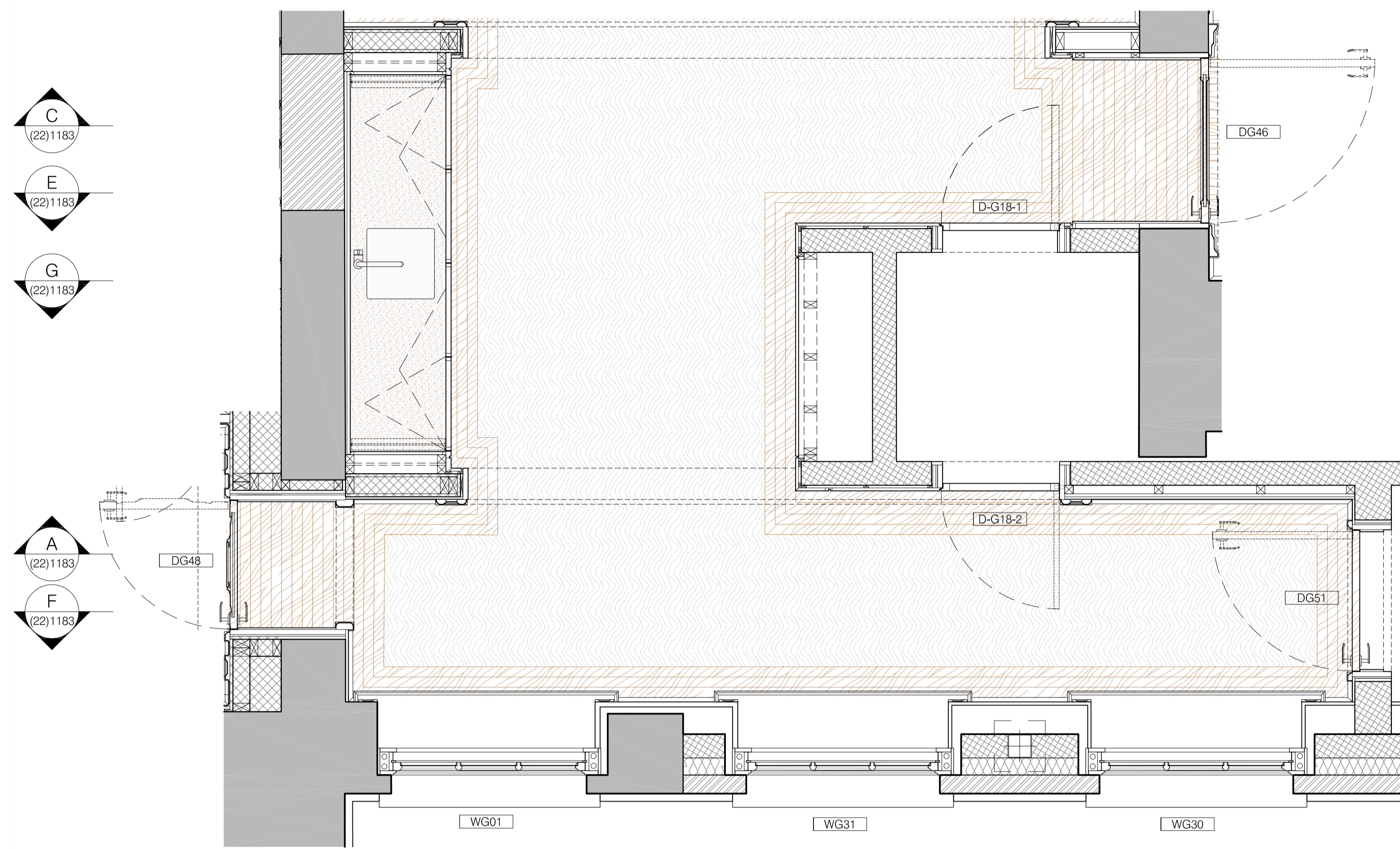
G18A SURVERY PLAN Scale: 1:20 @ A1
