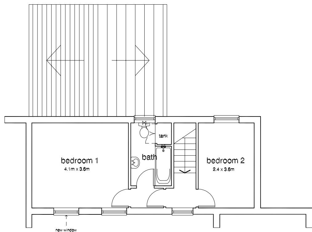
first floor as proposed
