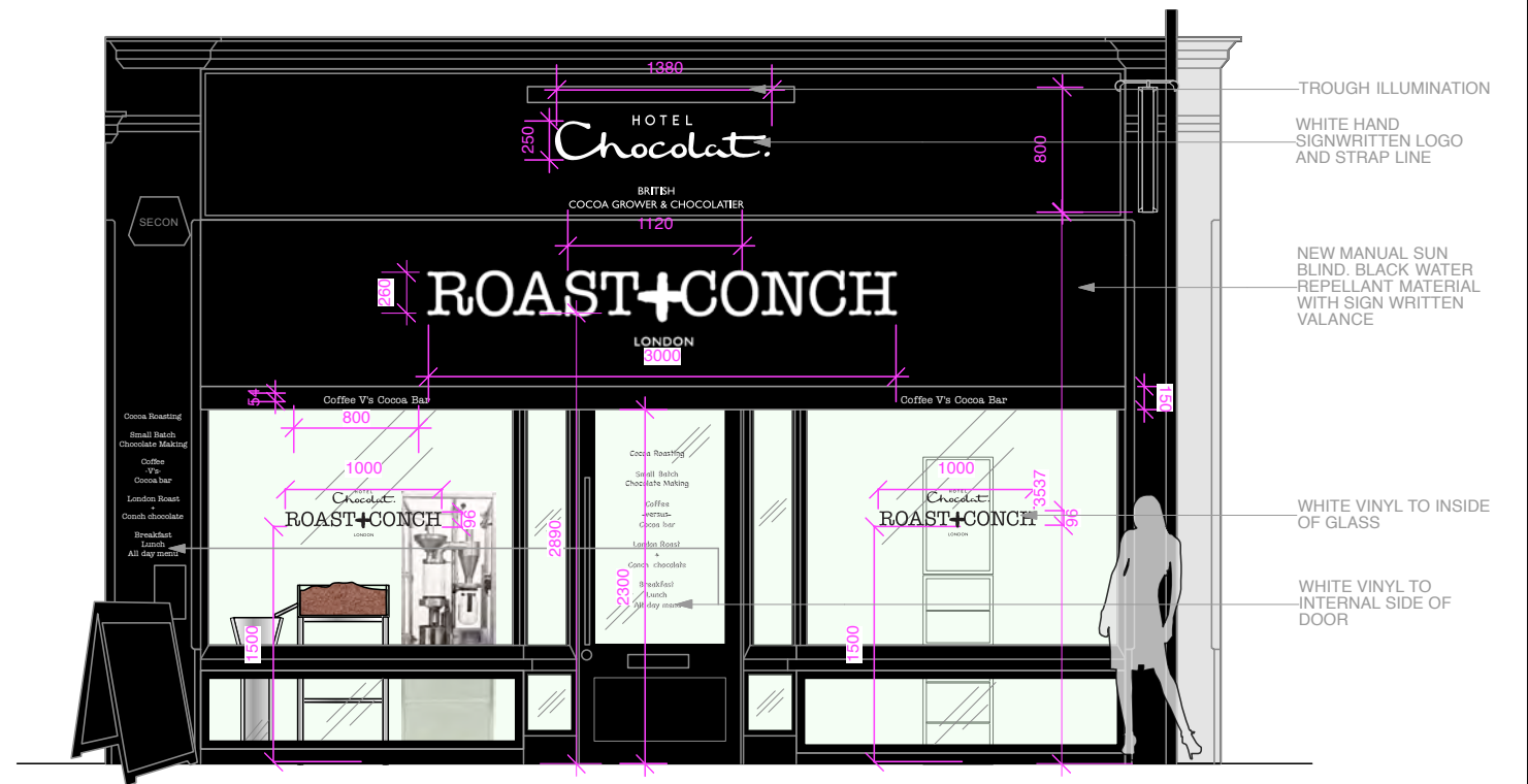
FRONT ELEVATION - BLIND OPEN SCALE @ 1:50
