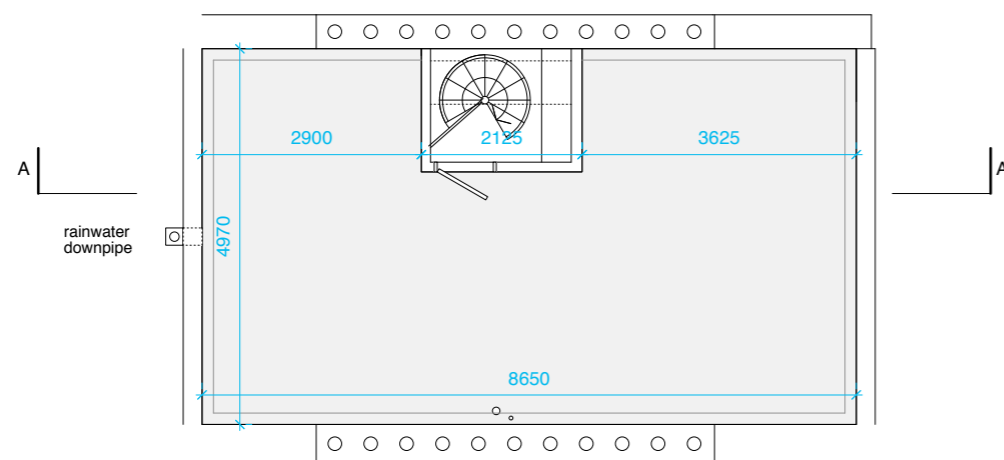
ROOF TERRACE PLAN
