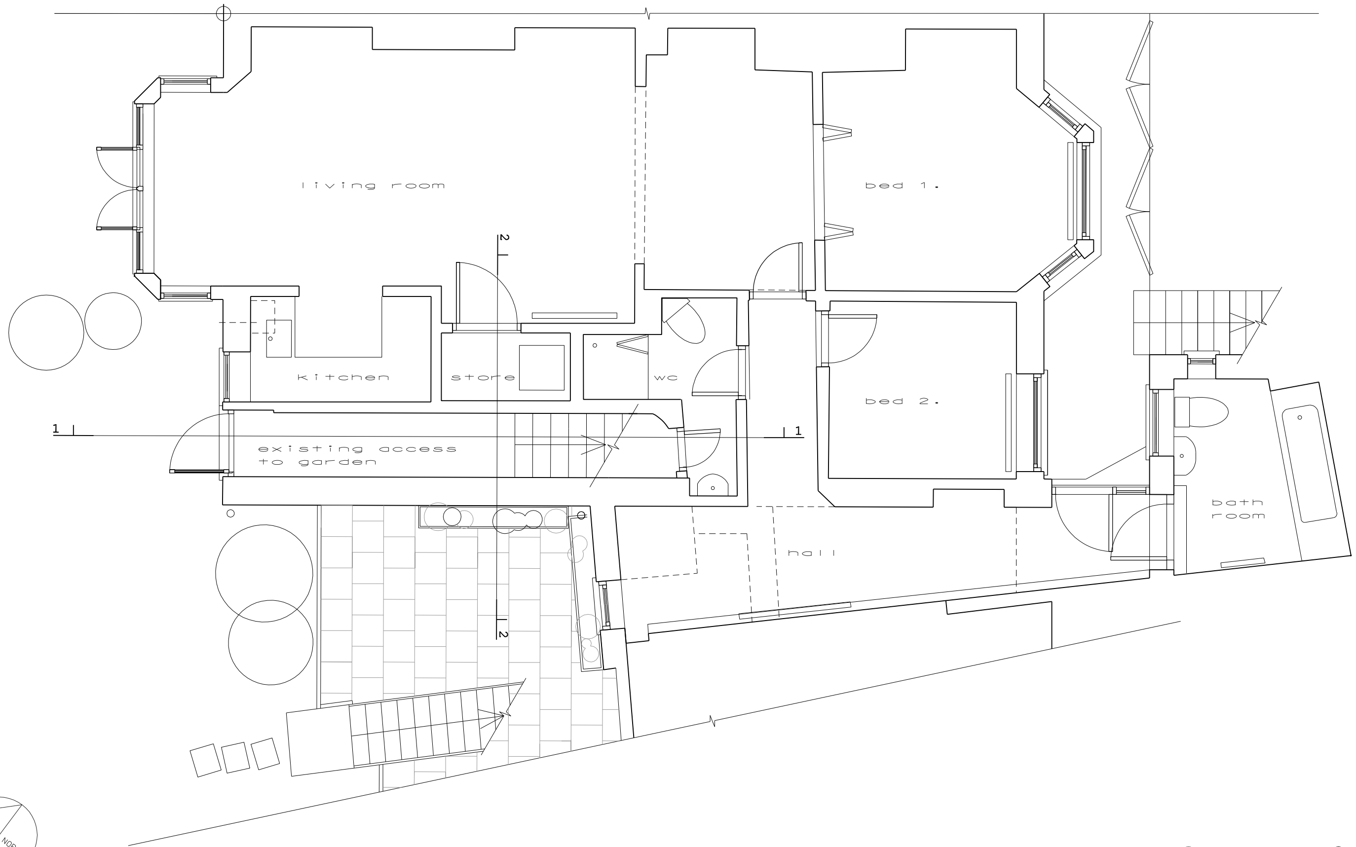
EXISTING LOWER GROUND FLOOR PLAN
