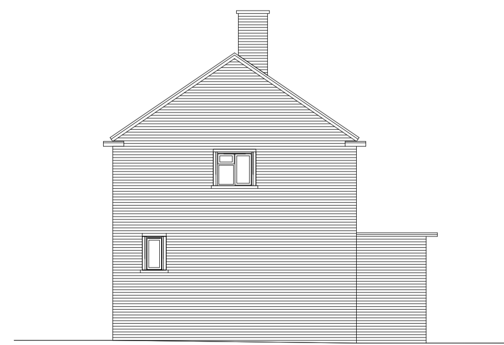
SOUTHEAST (SIDE) ELEVATION
