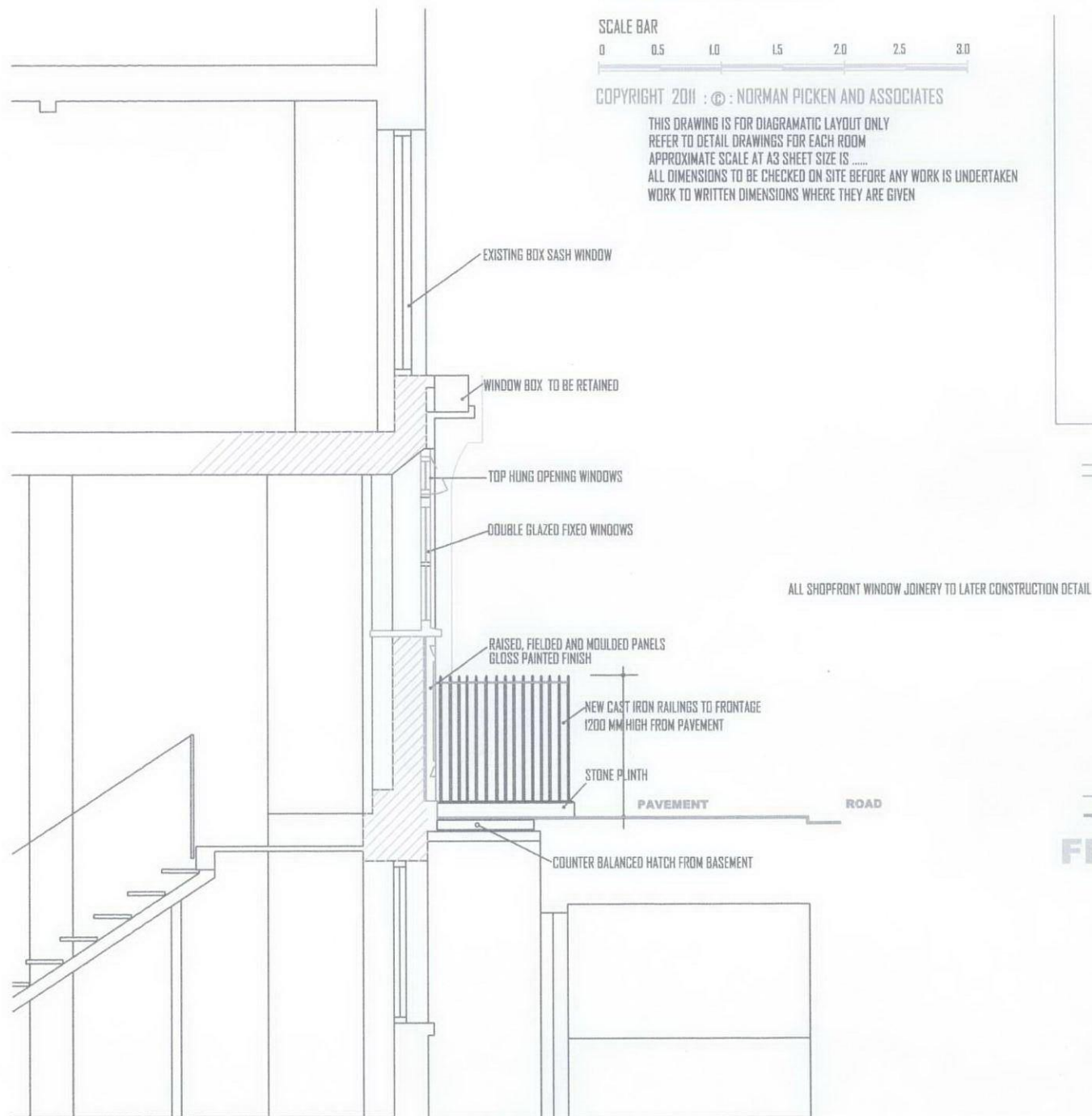
VERTICAL SECTION THROUGH PROPOSED FRONTAGE
