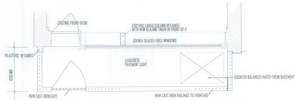
PLAN AS PROPOSED DECEMBER 2011
