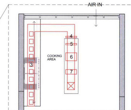
5 KITCHEN VENT - CEILING PLAN 1:100@A3
