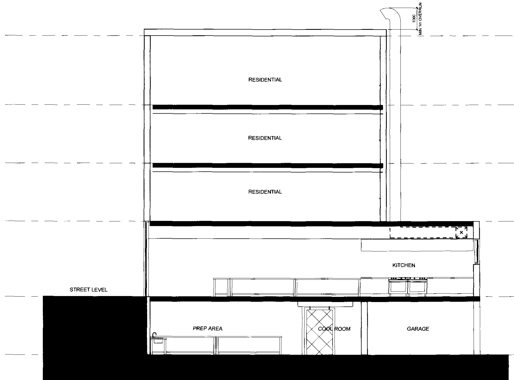
1 SECTION - PROPOSED 1:100@A3
