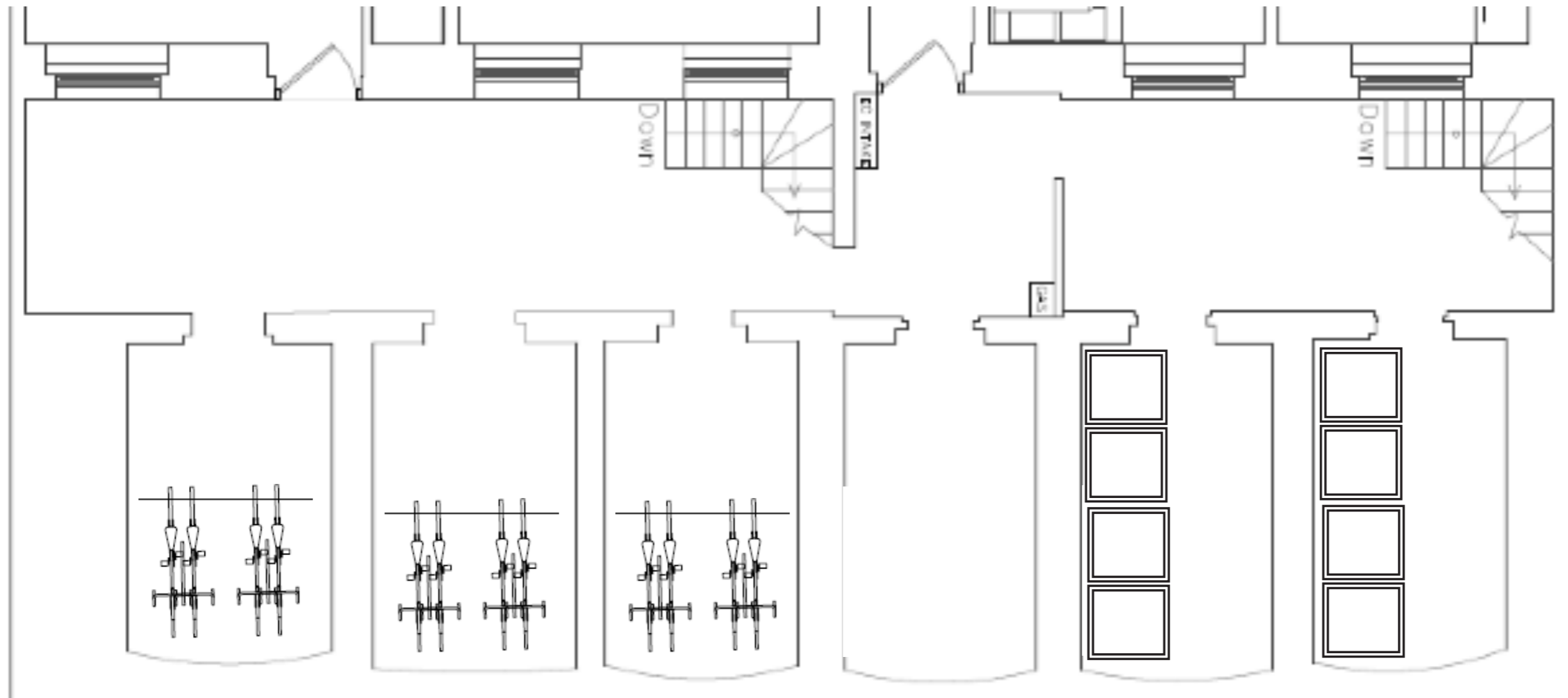
Cycle Storage 2 no. Sheffield Stands
