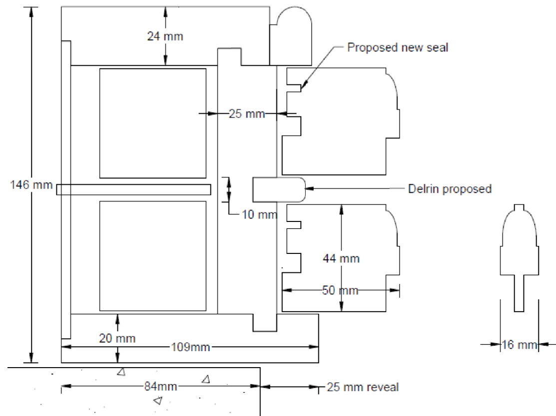
TYPICAL SASH WINDOW
