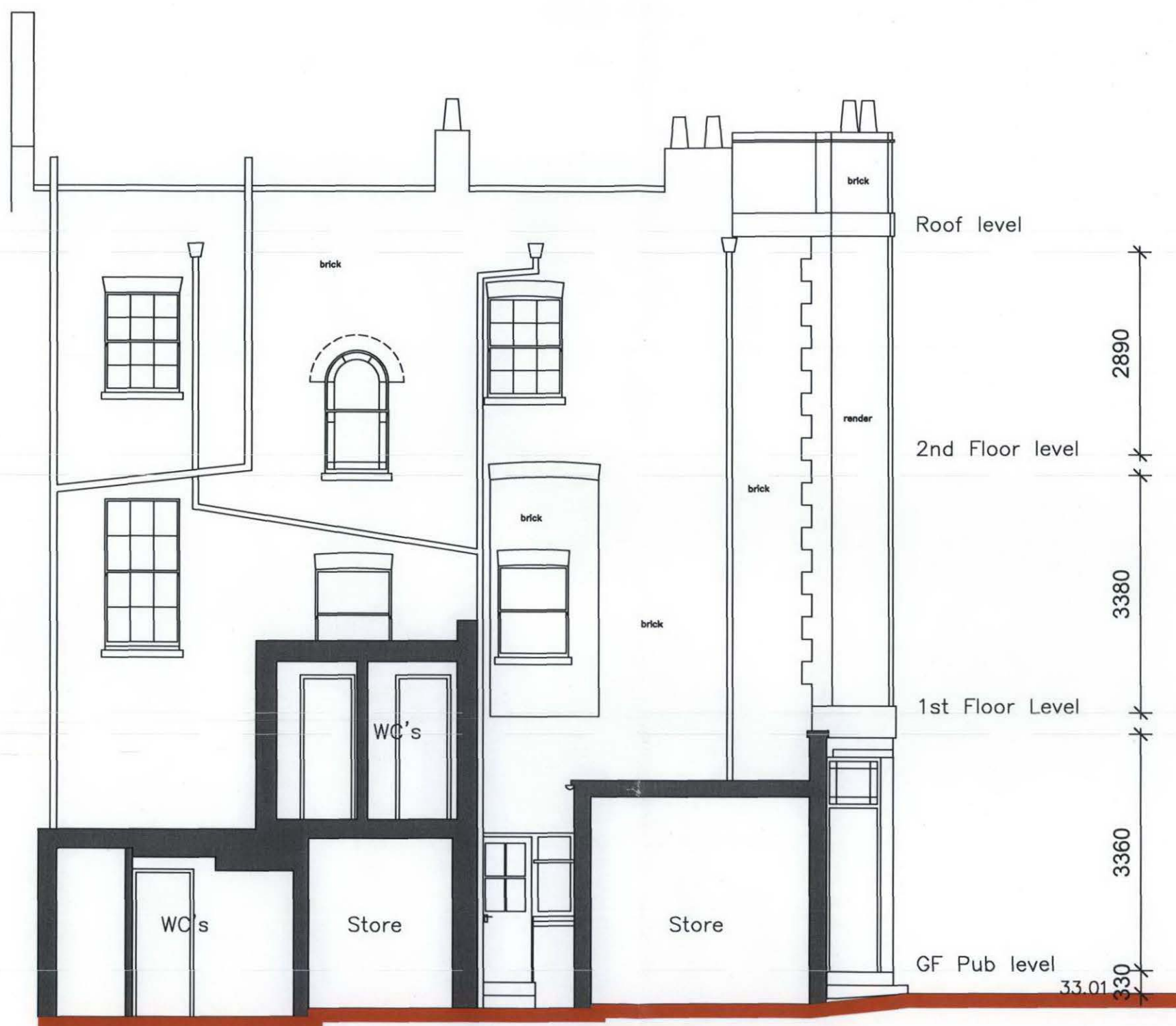
Existing South West Elevation/Section A-A
