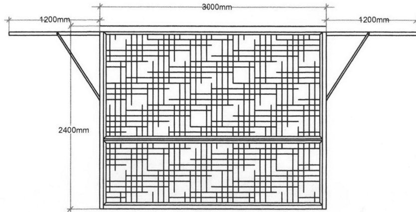
Side Elevation 1:50
