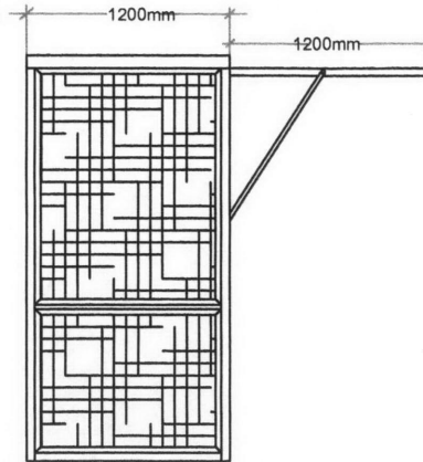
Side Elevation Open 1:50
