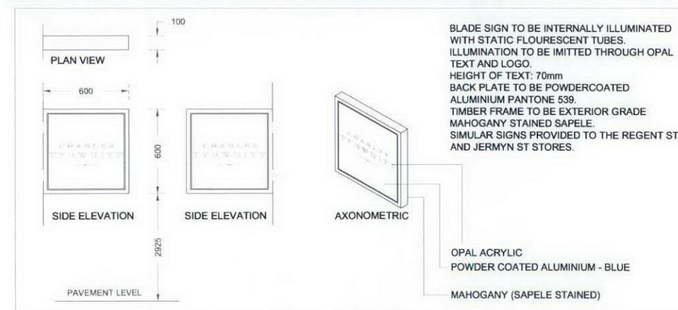
PROPOSED PROJECTING ILLUMNITED SIGNAGE.
