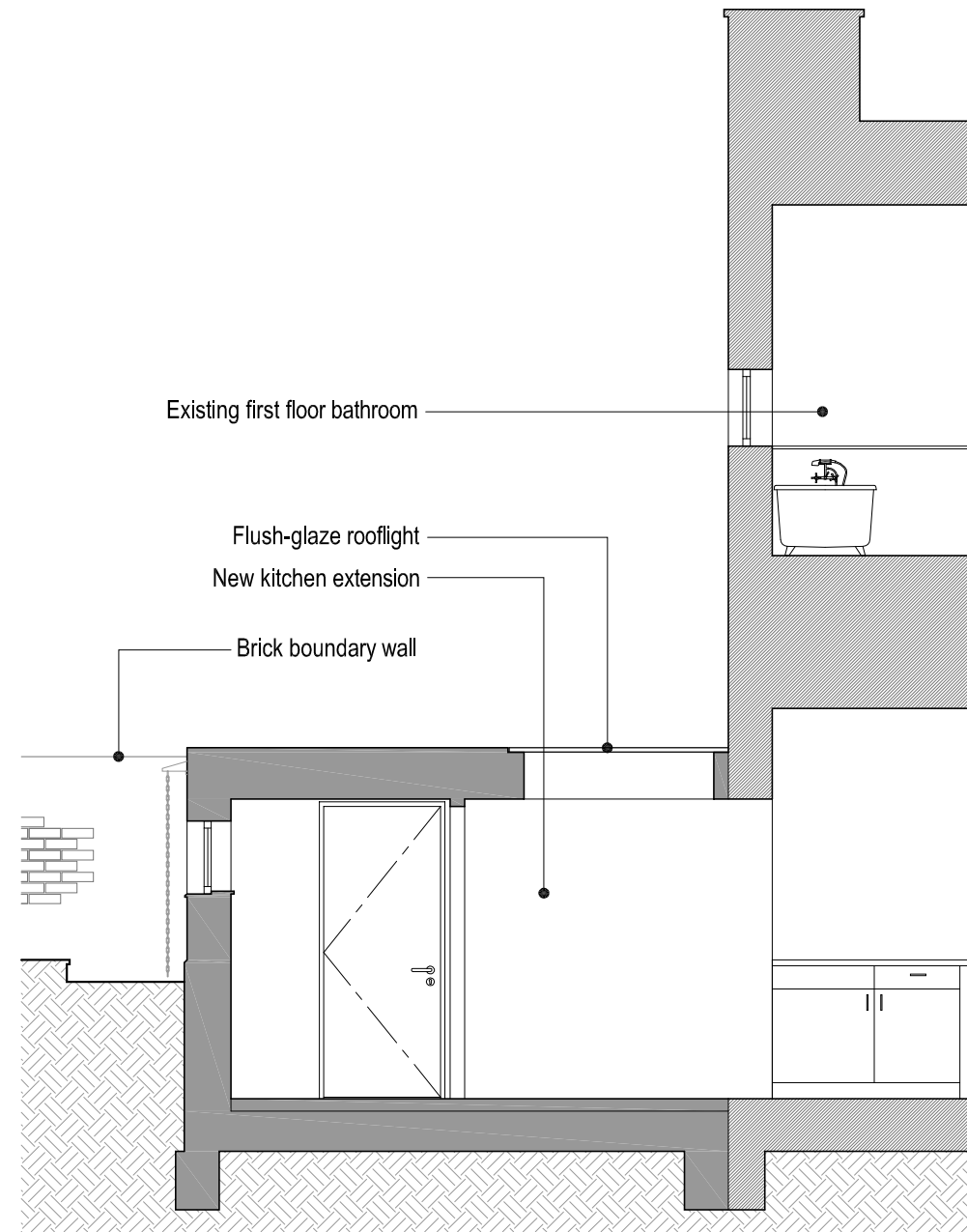
PROPOSED SECTION C-C
