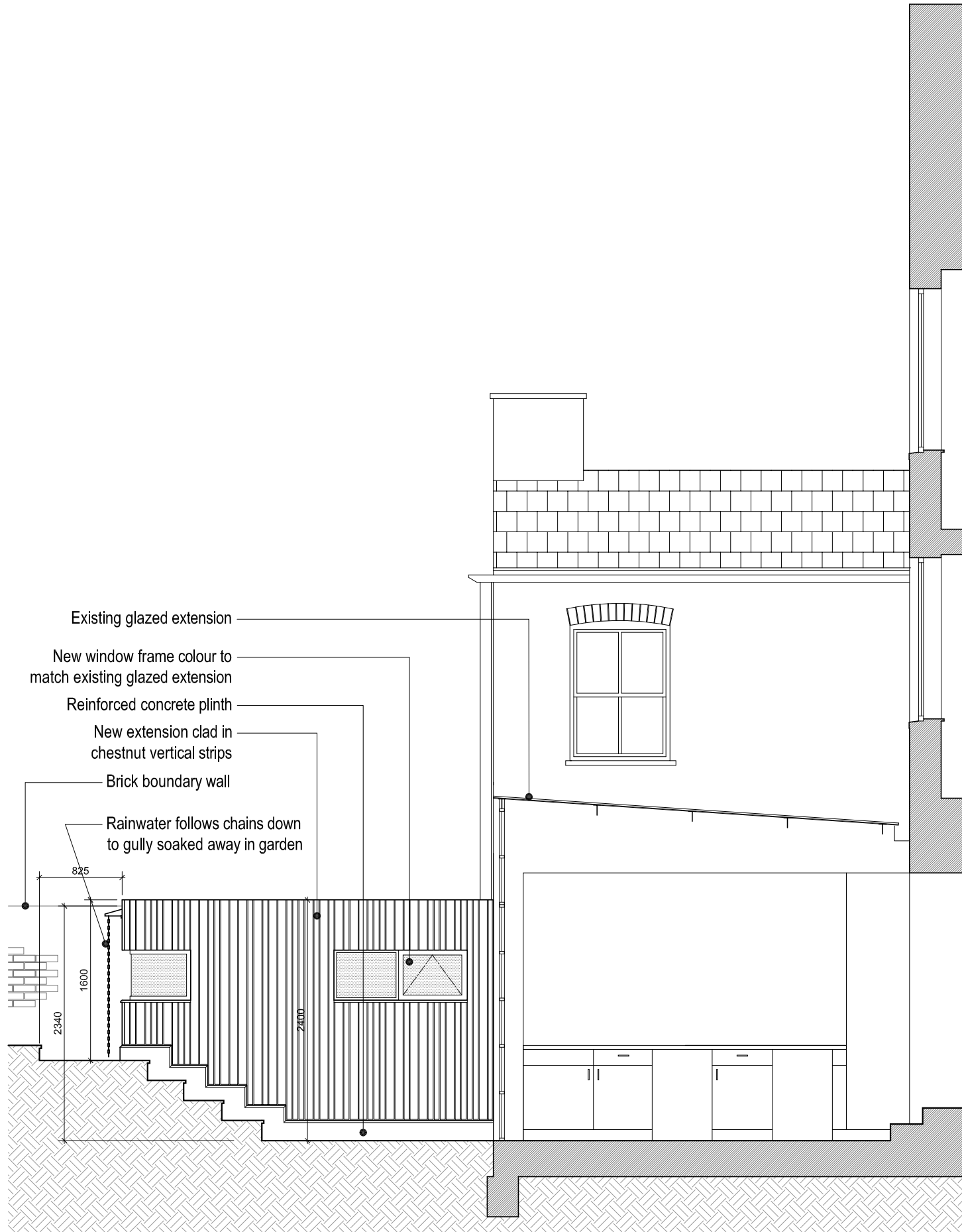
PROPOSED SECTION B-B
