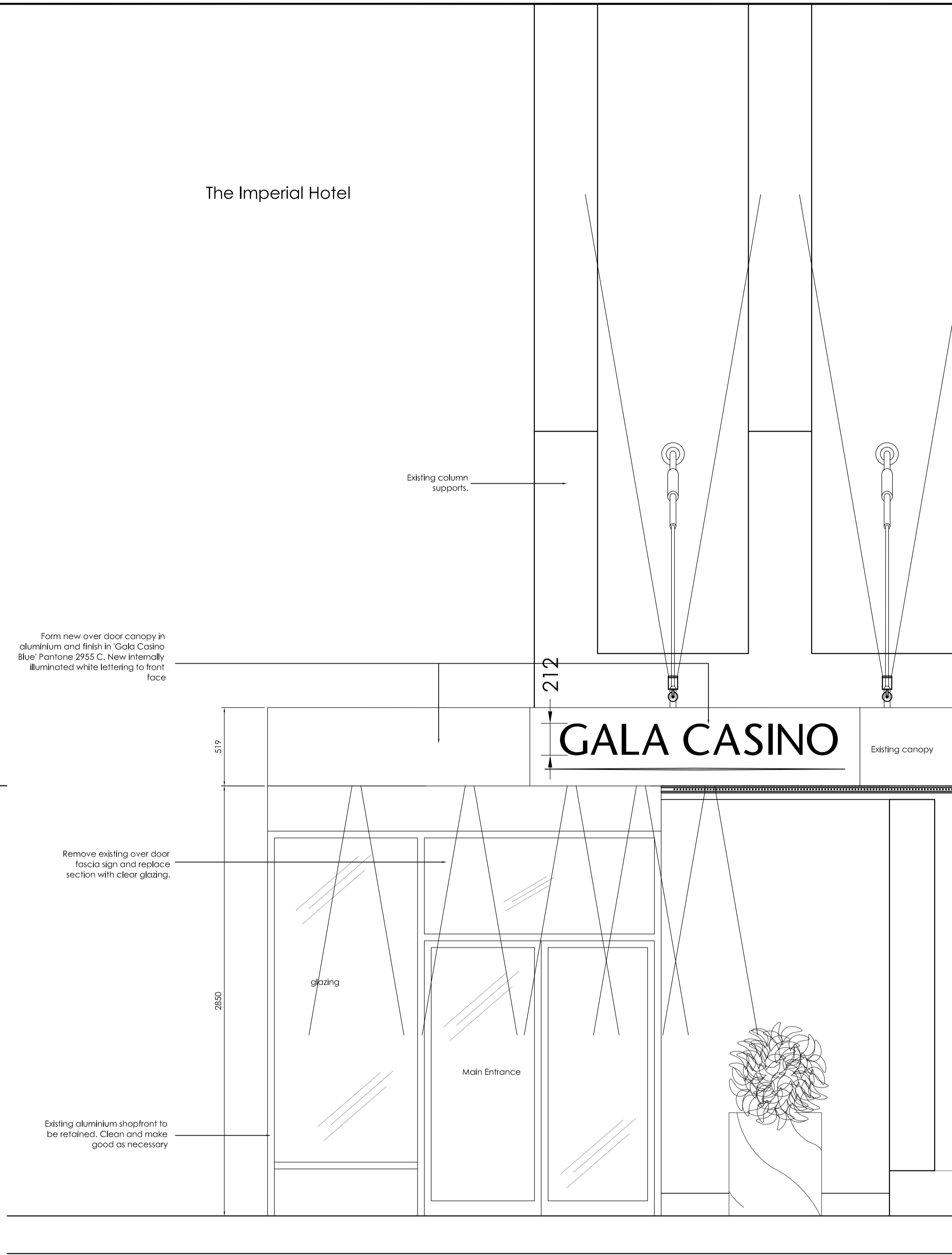
PROPOSED ENTRANCE CANOPY ELEVATION
