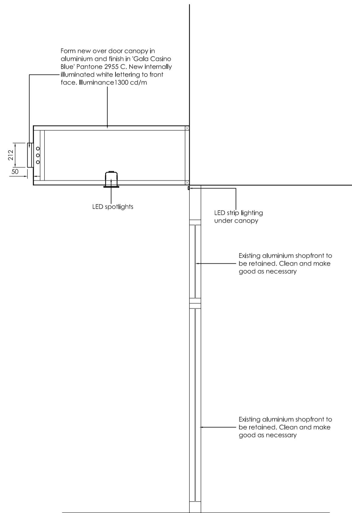
Section Thro' A-A
