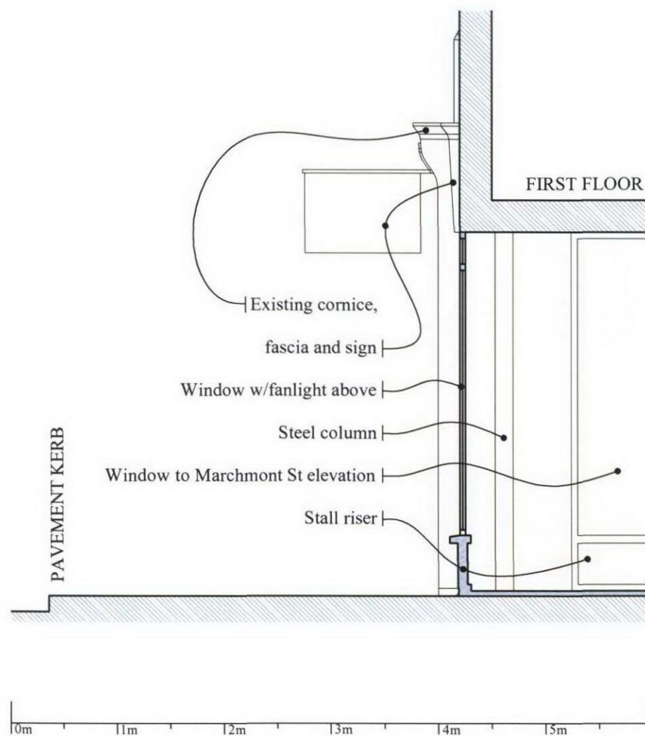
76 MARCHMONT STREET Section AA as Existing
