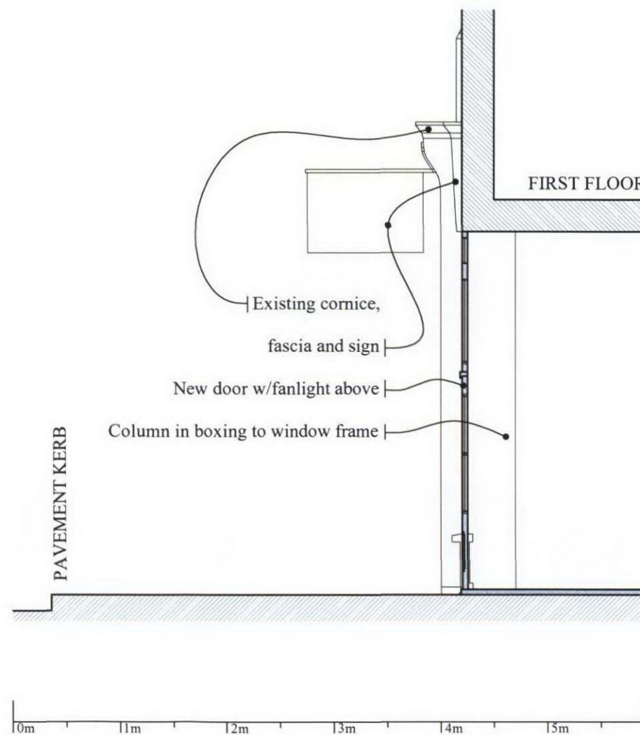
76 MARCHMONT STREET Section AA as Proposed
