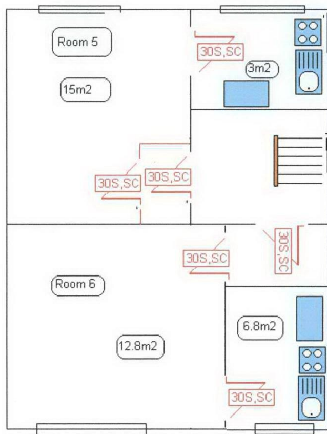
31 Agar Grove First Floor Layout
