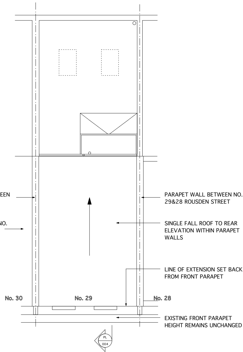
ROOF PLAN
