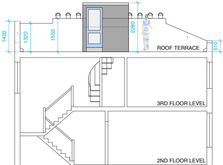
SECTION AA / EAST ELEVATION
