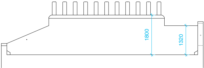
SECTION / WEST ELEVATION
