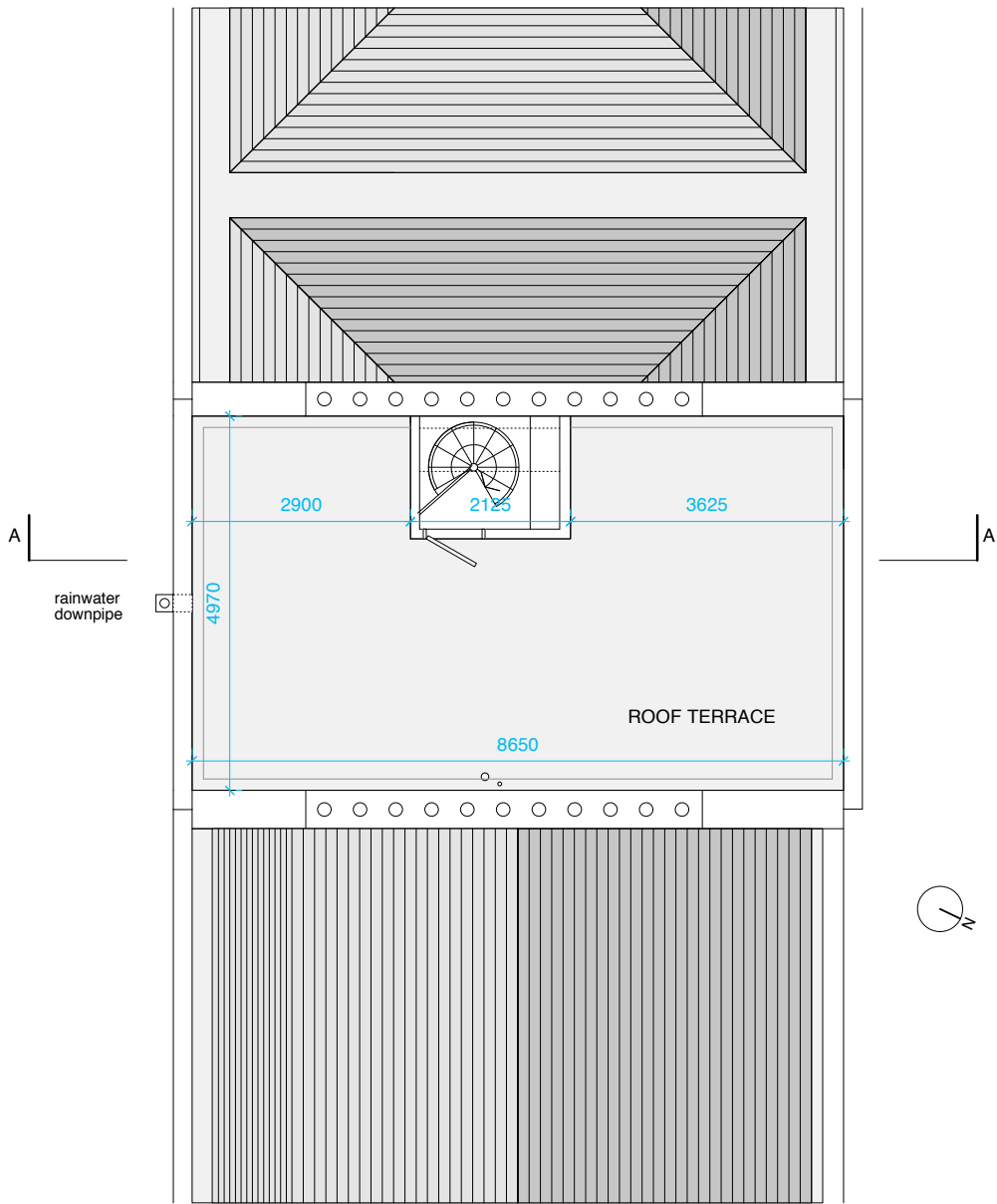
ROOF TERRACE PLAN
