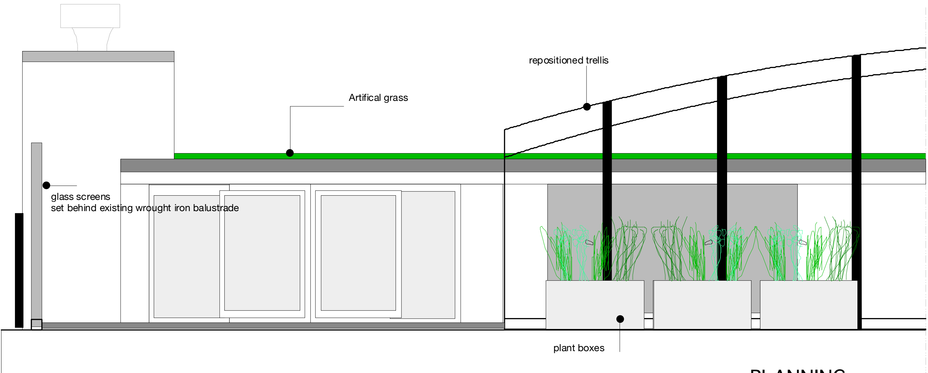
PROPOSED PART CROSS ELEVATION SHOWING NEW TRELLIS POSTION ARTIFICIAL GRASS OVER STORAGE AND PLANT ROOF, END VIEW OF STEEL UPRIGHT FOR GLASS PANEL
