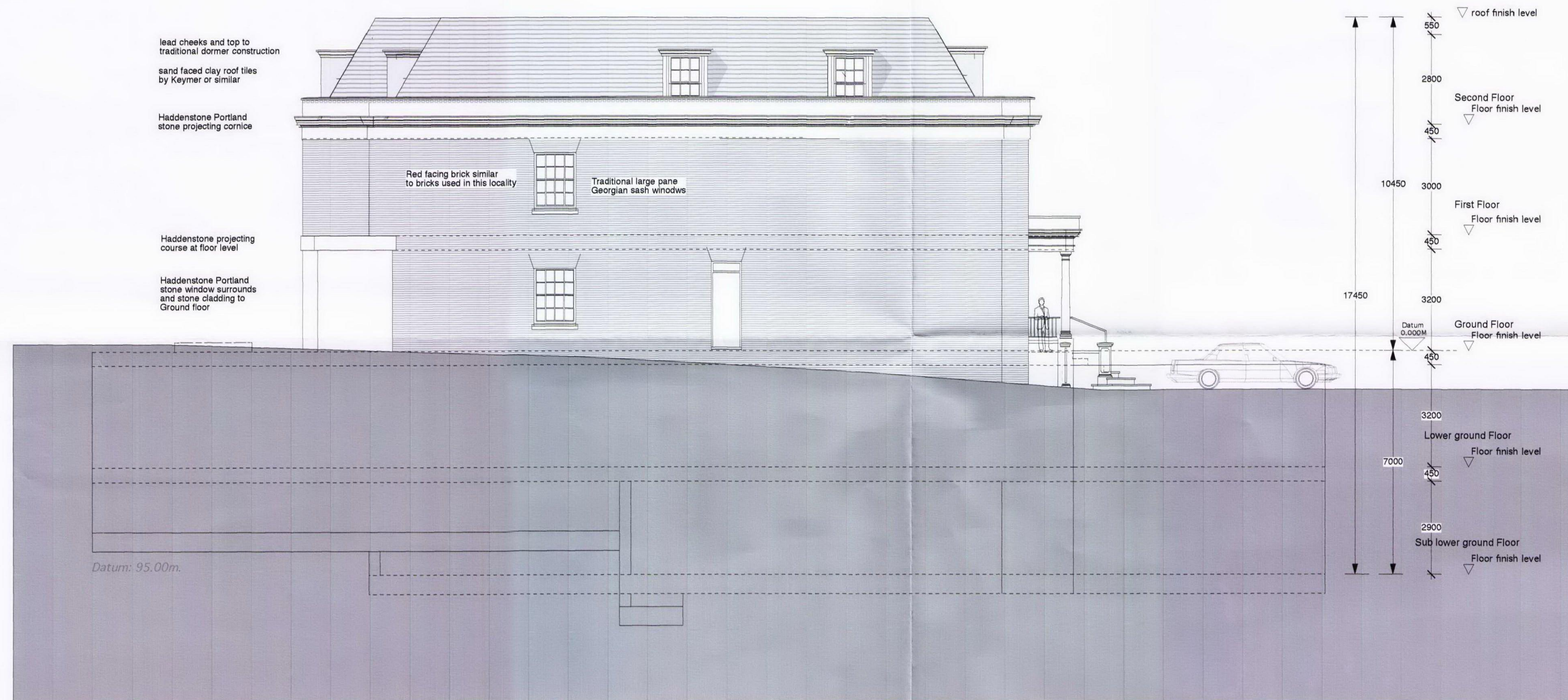
SIDE ELEVATION
