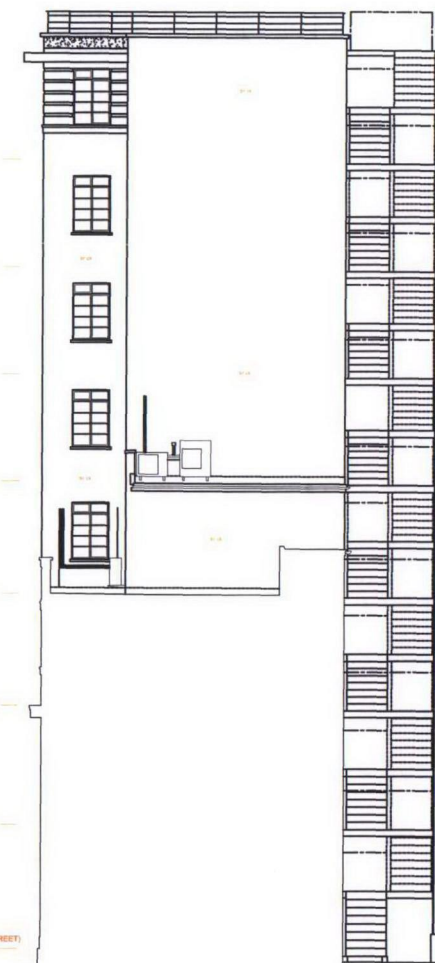
WEST ELEVATION
