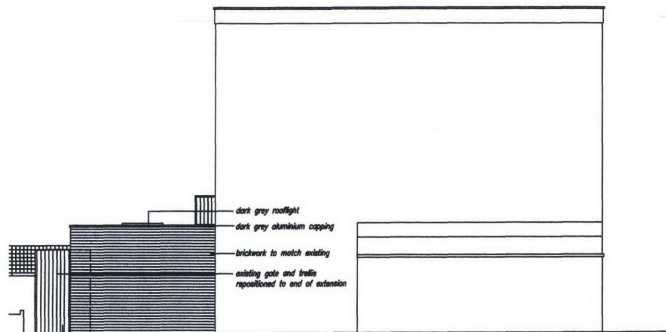
SIDE ELEVATION AS APPROVED
