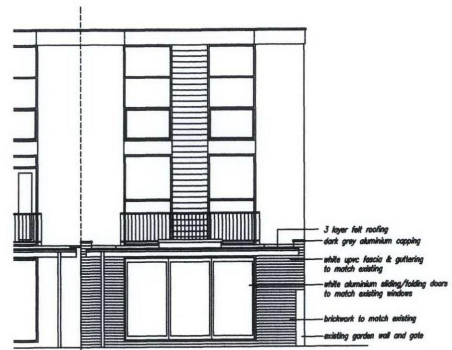
REAR ELEVATION AS APPROVED
