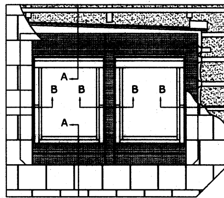
001 INDICATIVE LOCATIONS OF DETAILS
