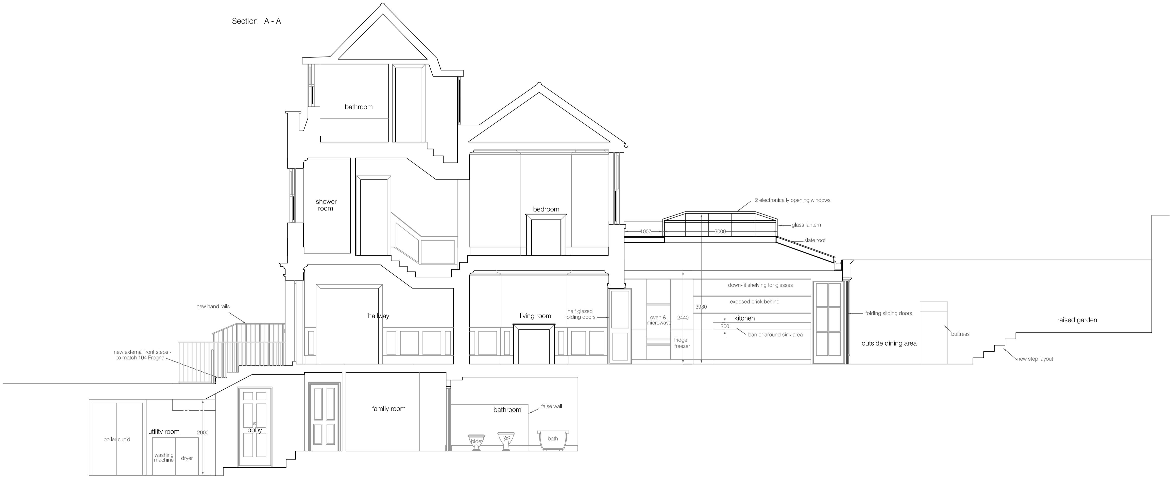
Section B - B
