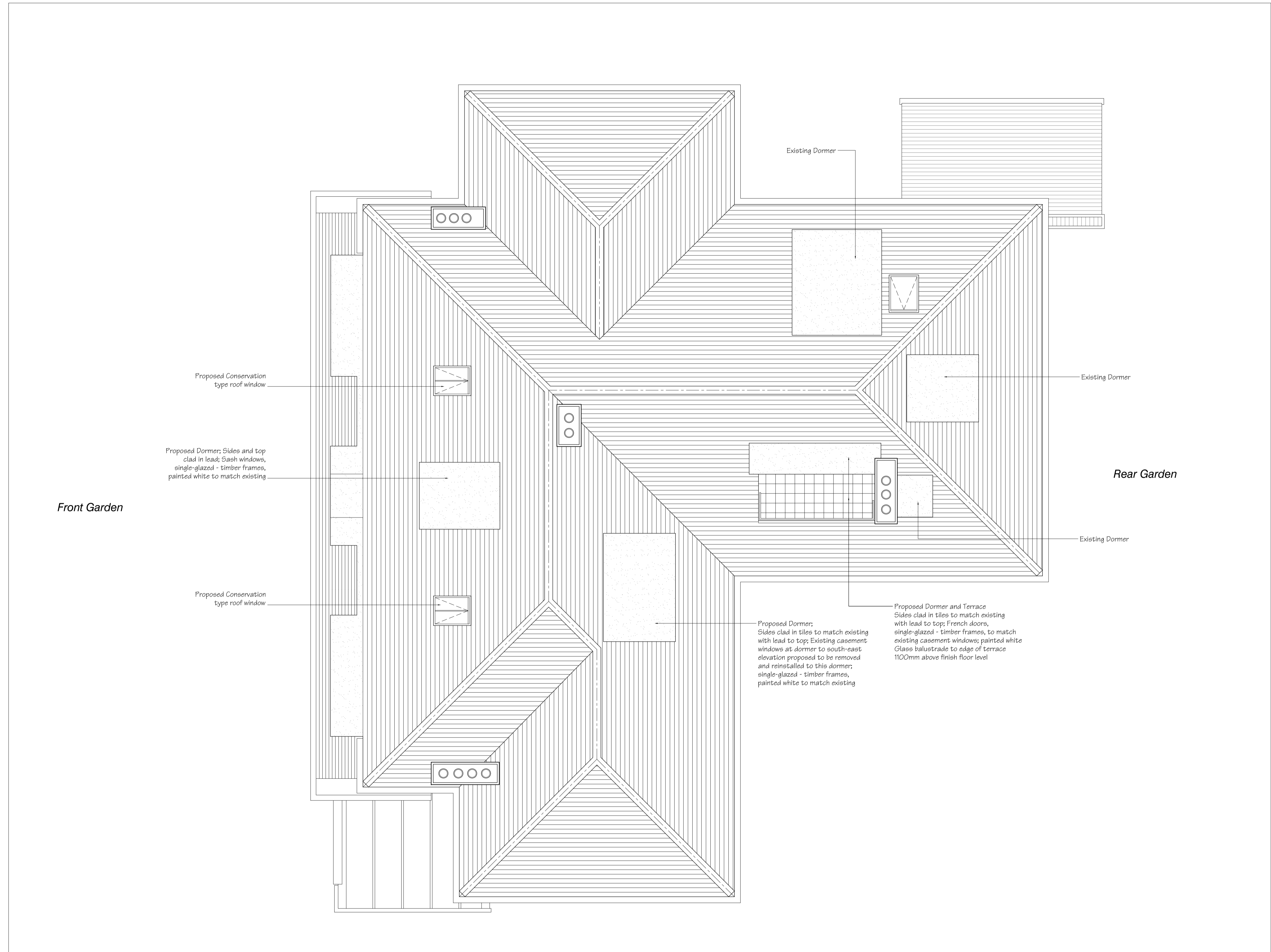
Proposed Roof Plan Scale 1:50 @A1
