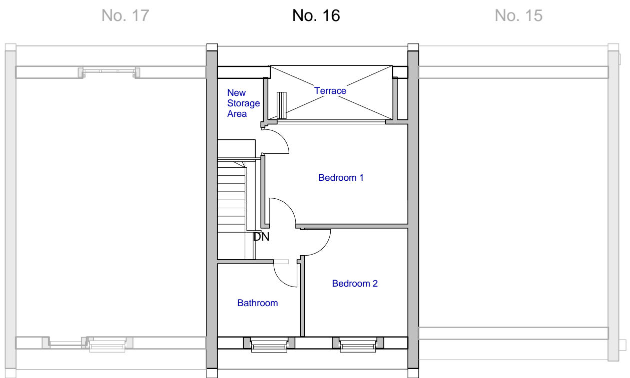
3rd Floor Plan - Proposed
