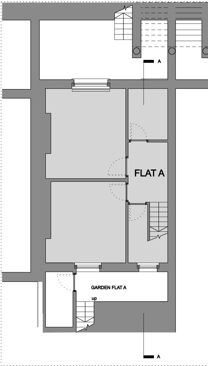
BASEMENT PLAN
