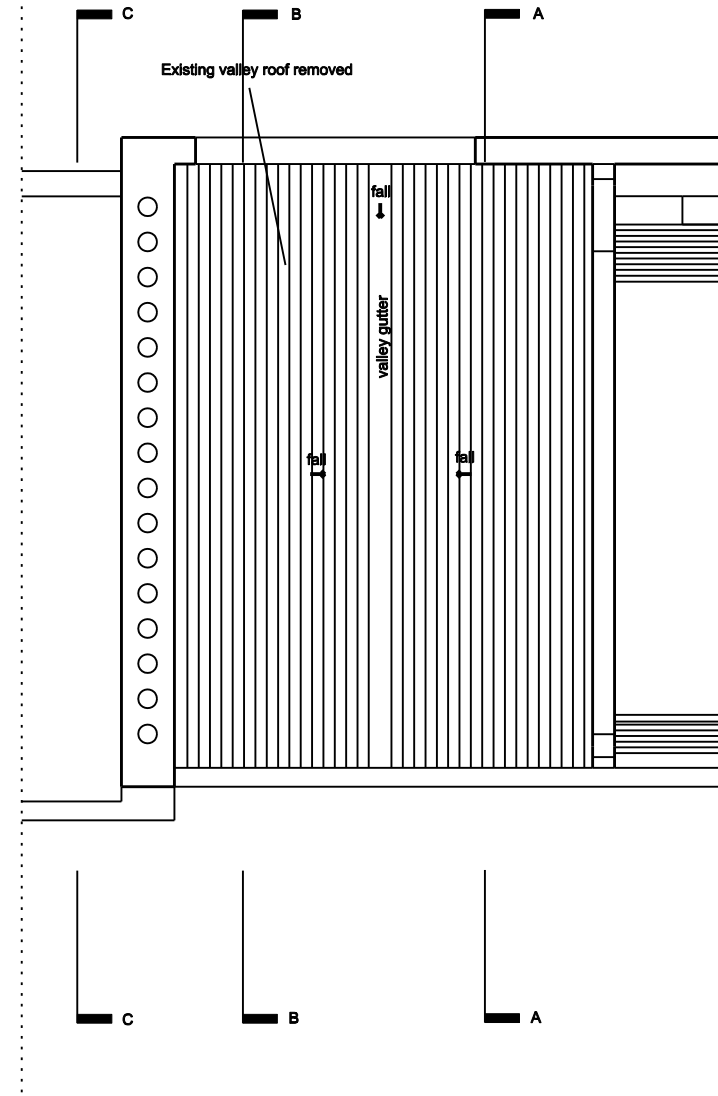
ROOF PLAN 1:100
