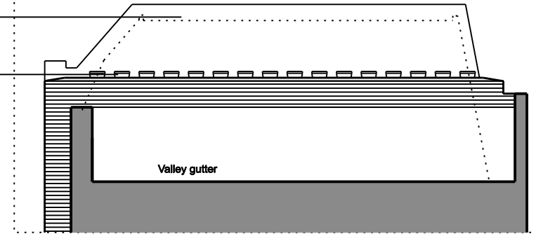
EXISTING SECTION C C
