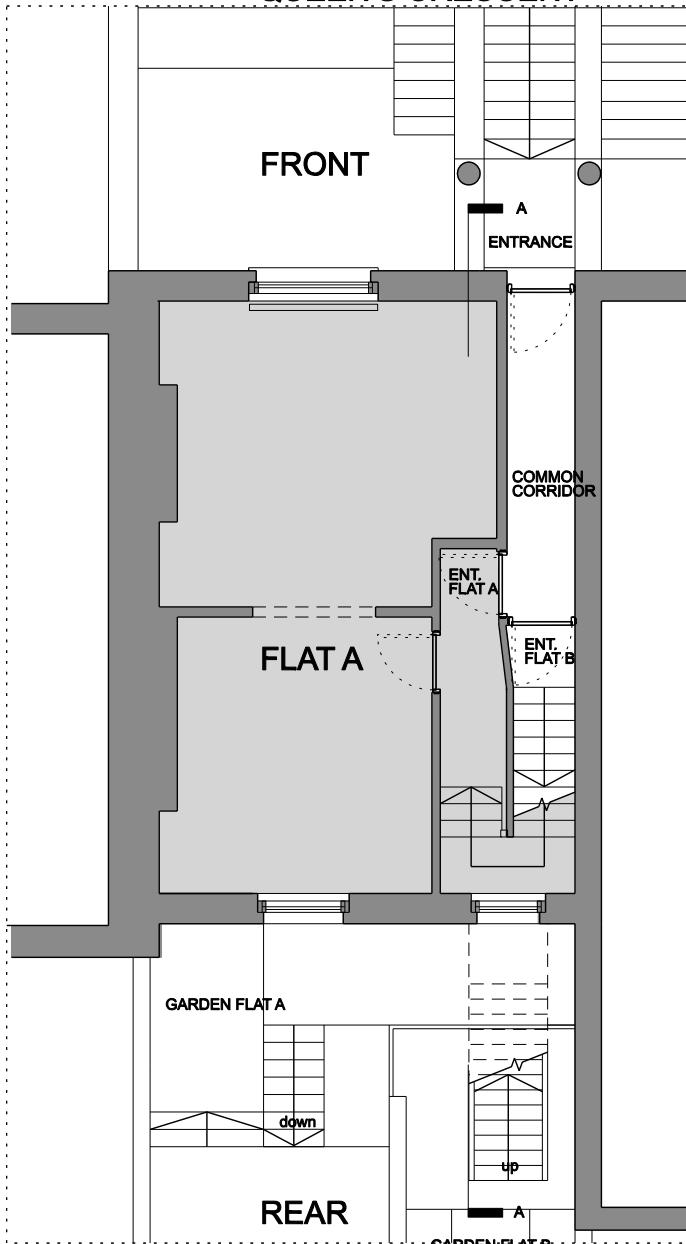
GROUND PLAN
