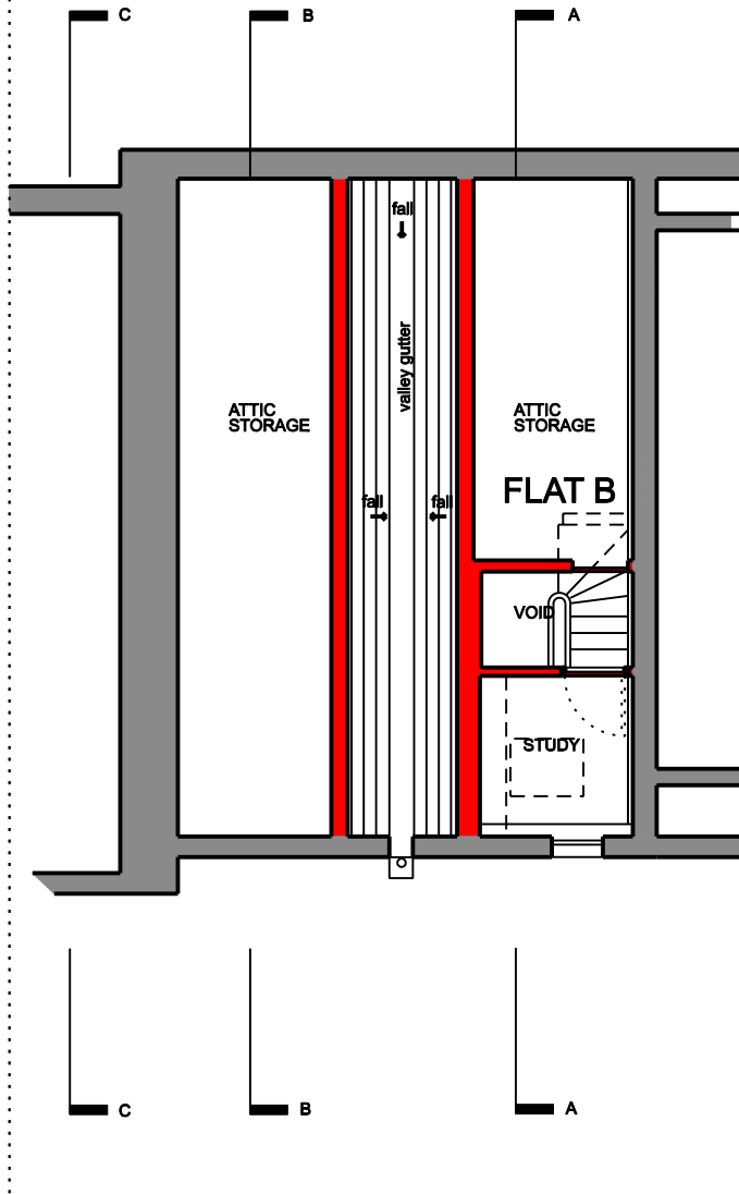
ATTIC PLAN 1:100
