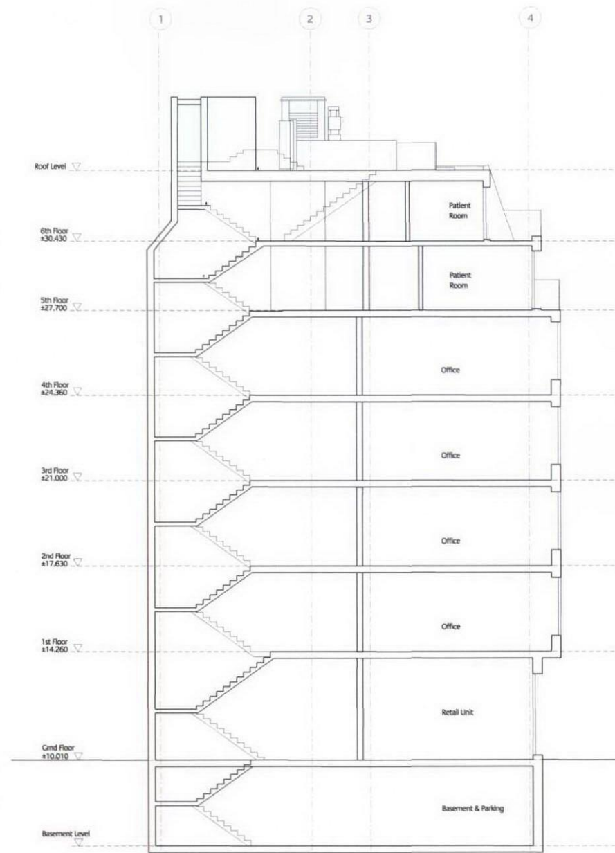
EXISTING SECTION A-A
