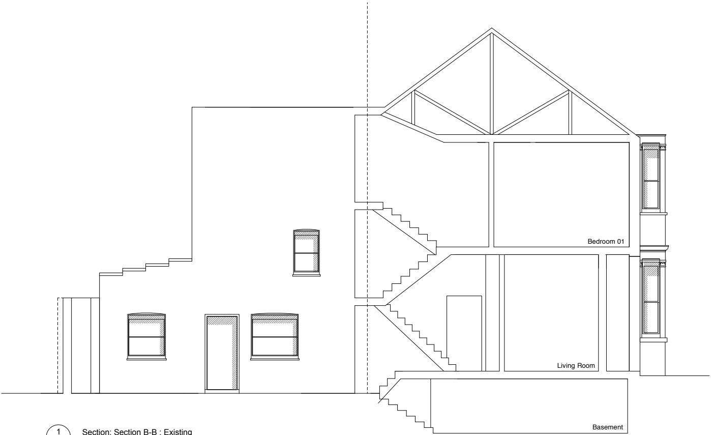
1 103 Section: Section B-B : Existing Scale: 1:100 @ A3
