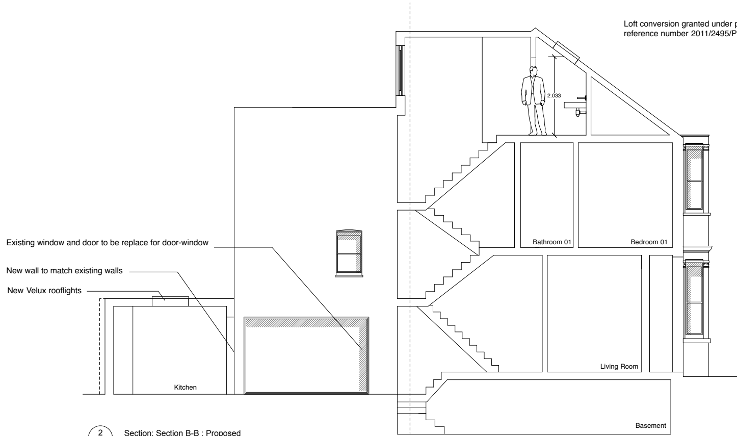
2 103 Section: Section B-B : Proposed Scale: 1:100 @ A3
