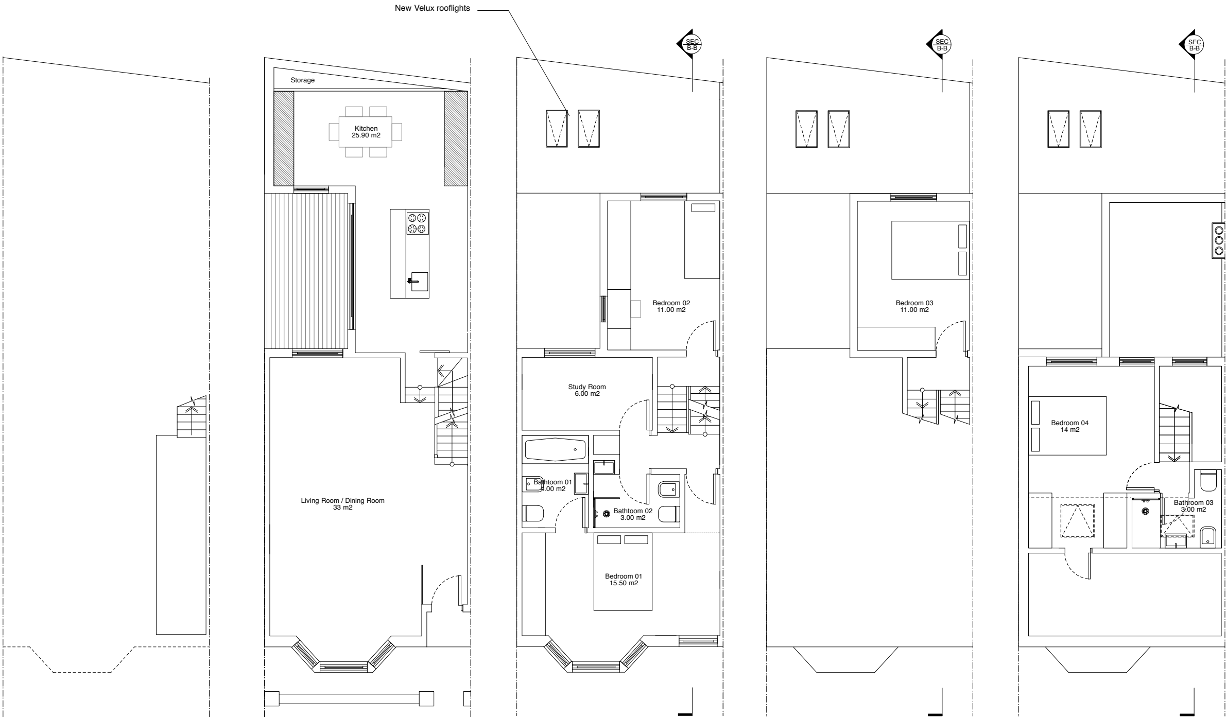
1 102 Plan: Basement Floor Plan : Proposed Scale: 1:100 @ A3
