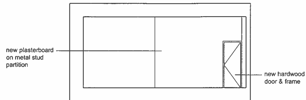
View CC
